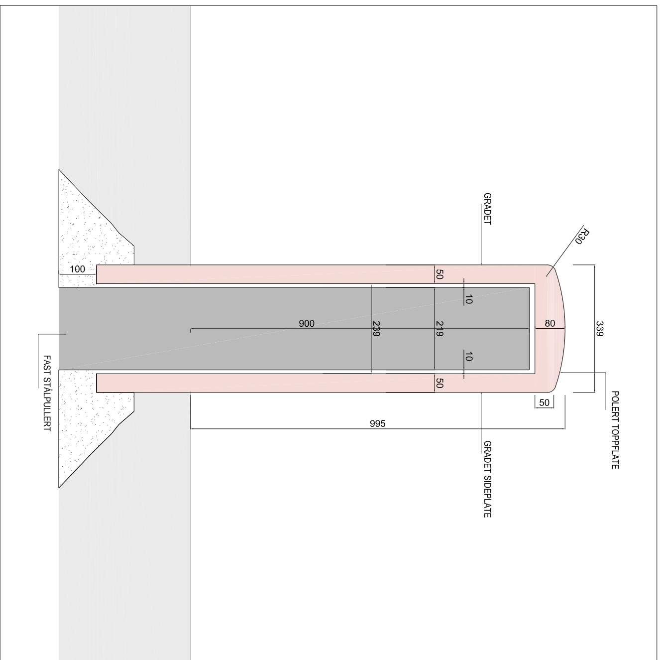
SNITT (1:10)
