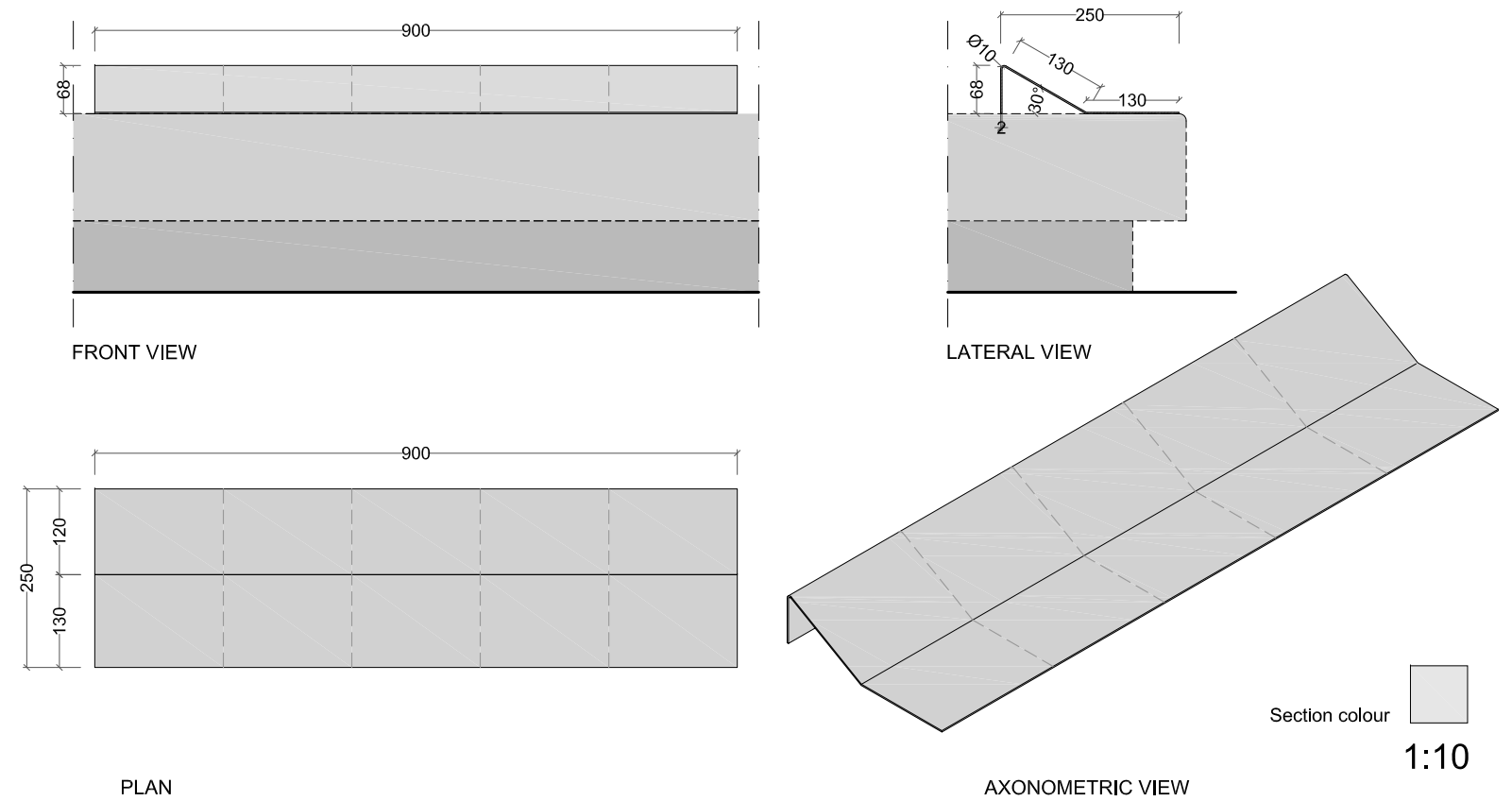
LH_T1-H260L900
