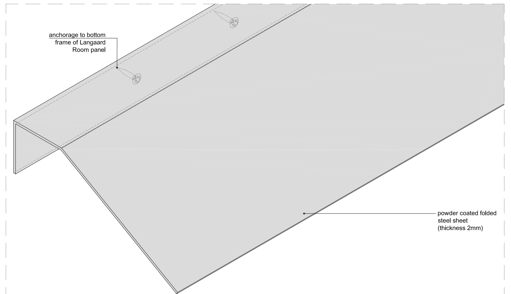
DETAIL 2
