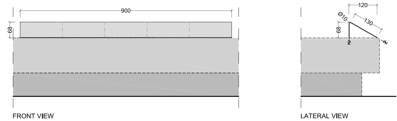
LH_T2-H130L900
