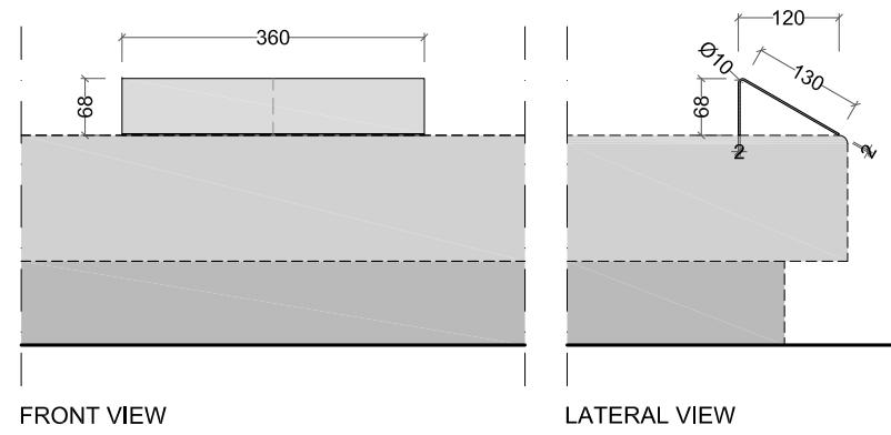
LH_T2-H130L360
