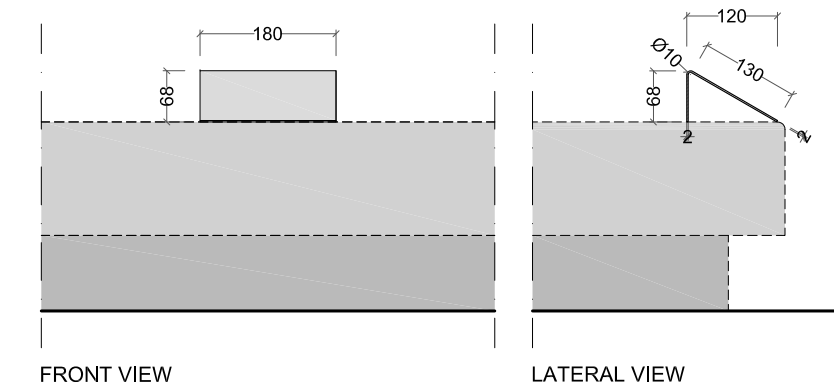
LH_T2-H130L180
