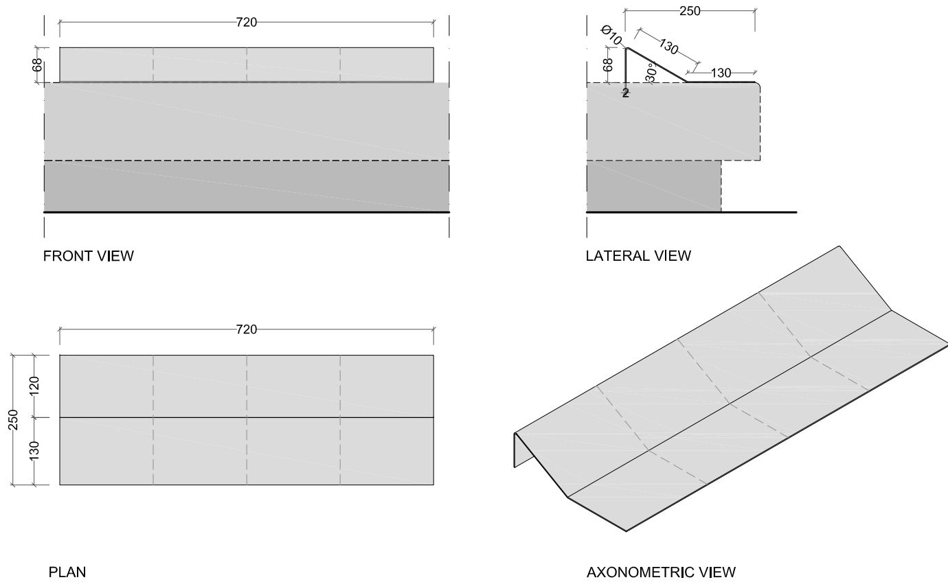
LH_T1-H260L720
