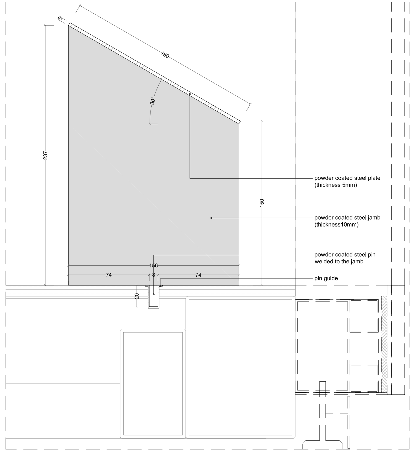
SECTION B
