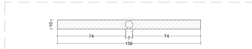
DETAIL 1
