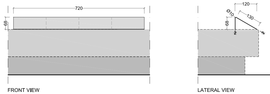
LH_T2-H130L720
