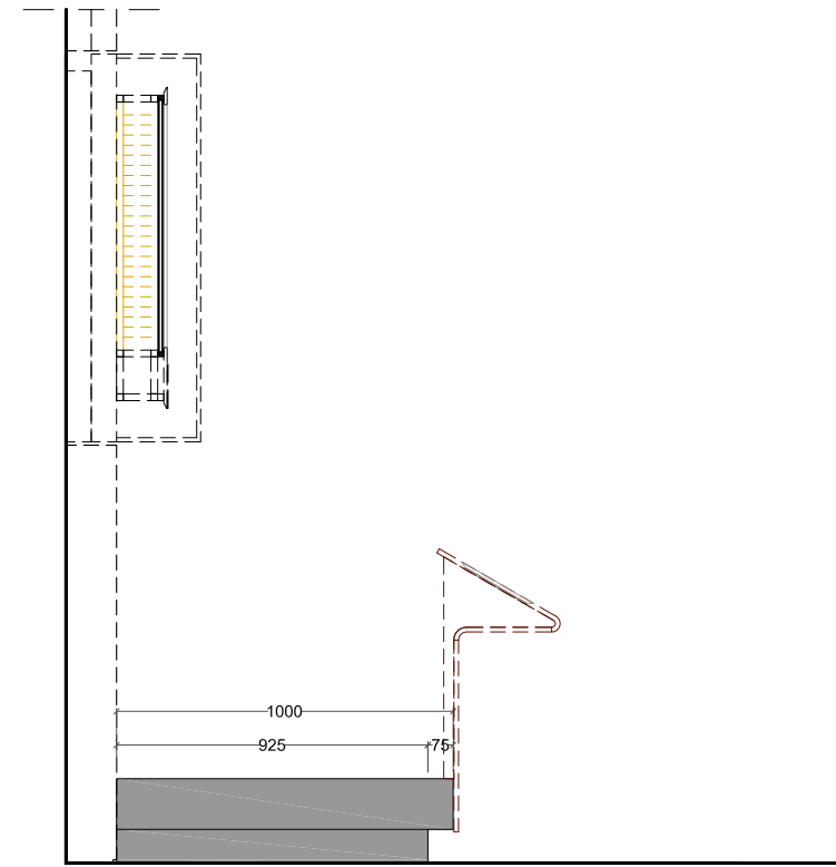
Side view
