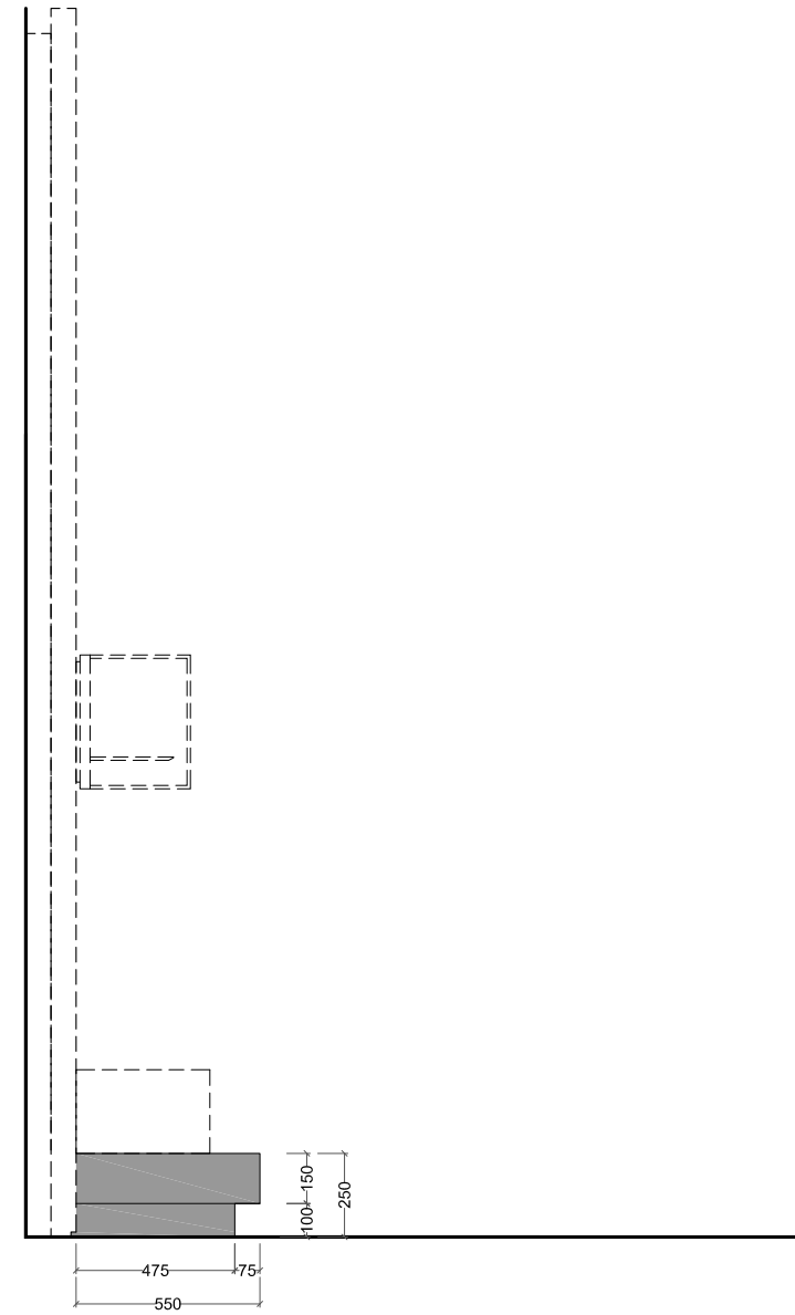
Side view
