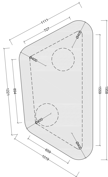
Plan
