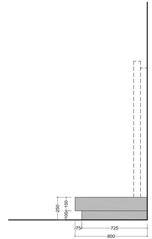
Side view
