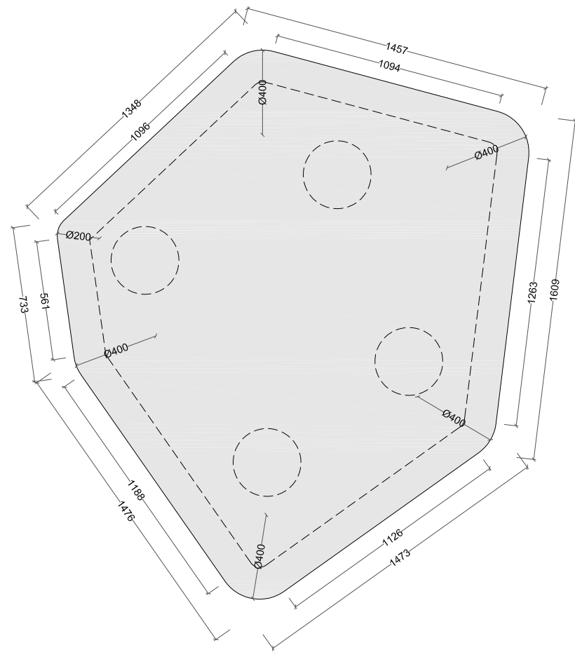
Plan
