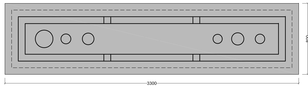
Plan
