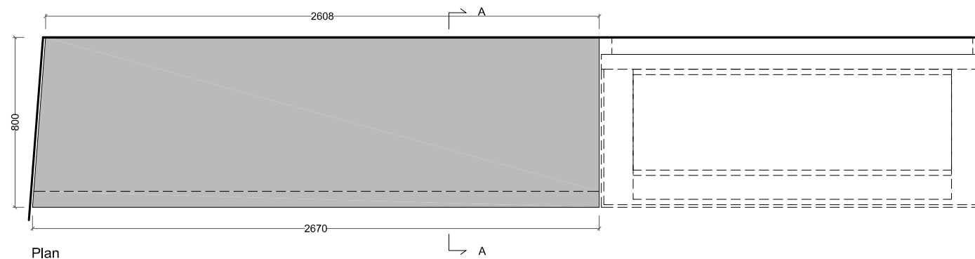
Plan
