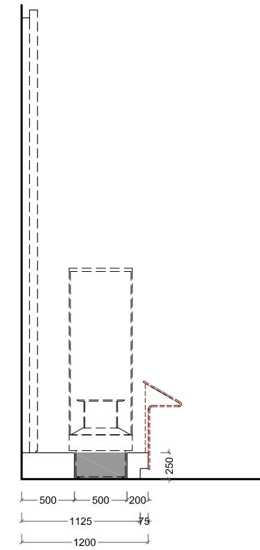
Section A
