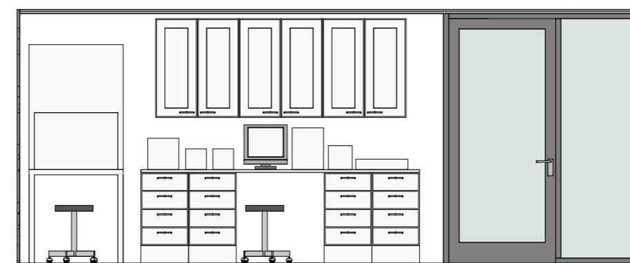
Quarantine materials - vegg C 1 : 50
