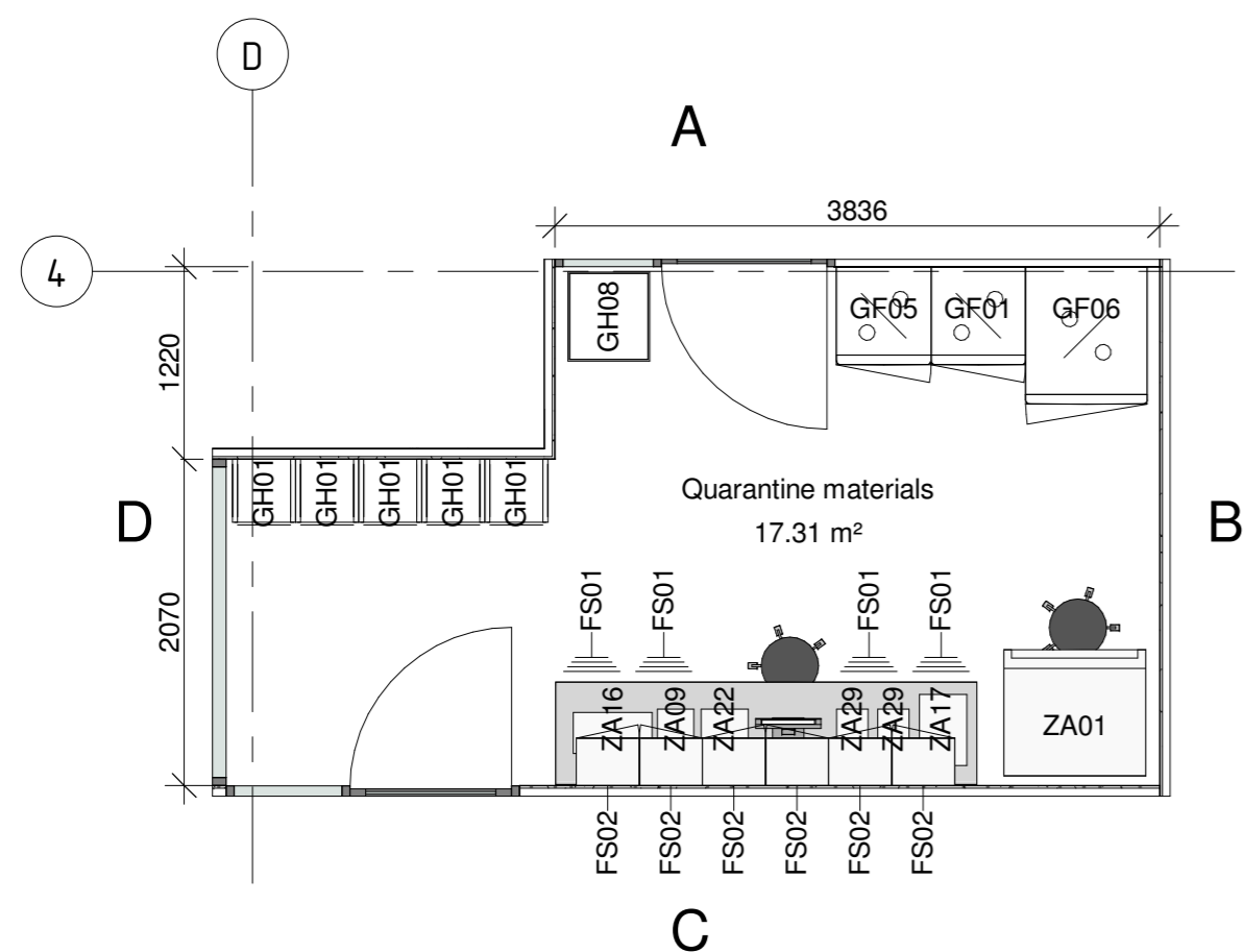
Plan Quarantine materials 1 : 50
