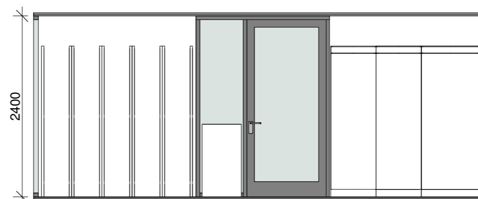
Quarantine materials - vegg A 1 : 50
