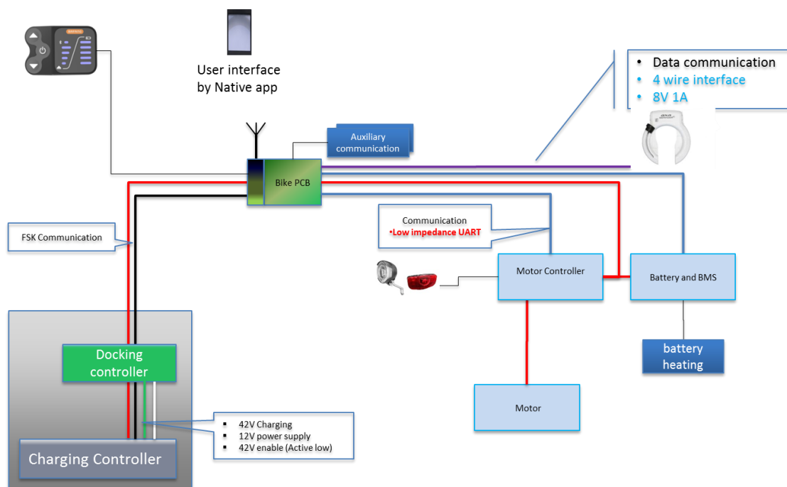
System schematics: Motor controller and Battery BMS may communicate to bikePCB via UART (as above) or via Auxiliary communication (CAN Bus or USB).
