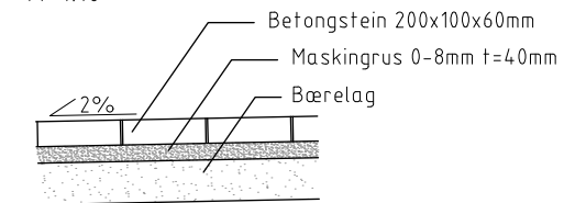
Snitt betongstein M=1:10
