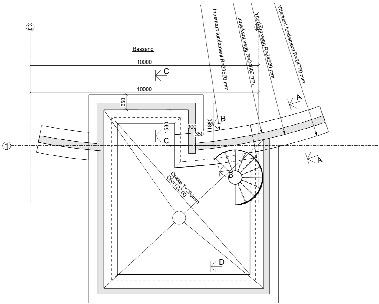
PLAN 122.00 1:50
