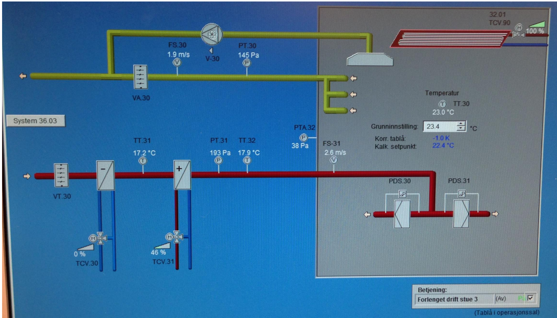
Bilde Desigo Insight system 36.03D OP3:
