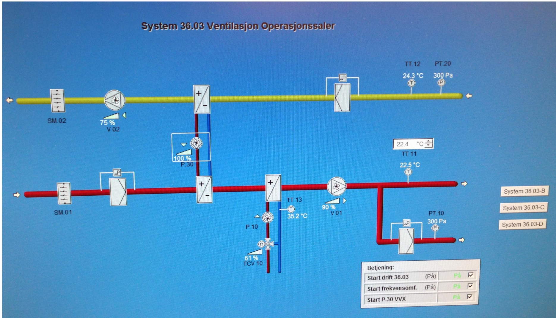
Bilde Designo Insight system 36.03:
