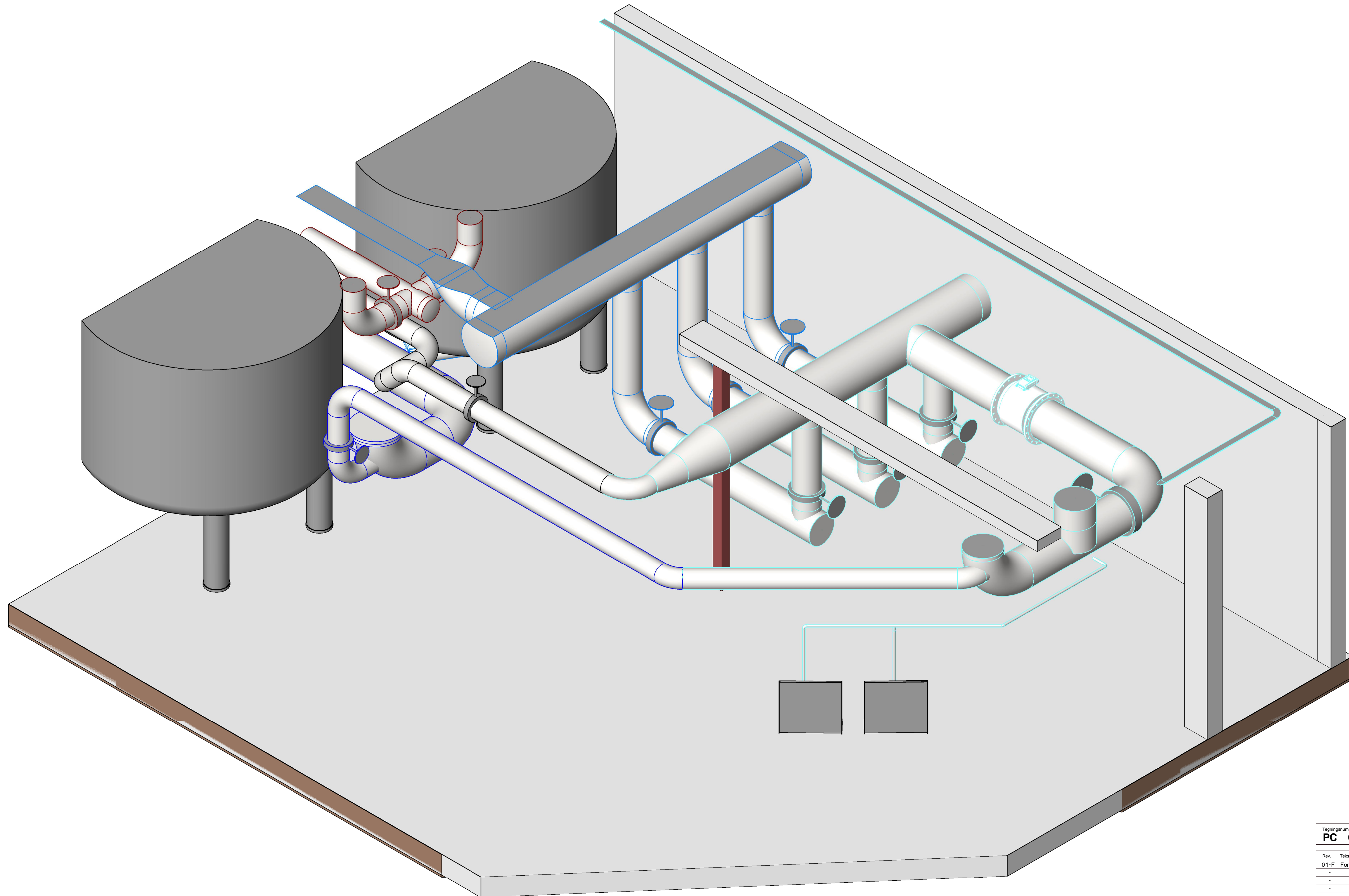
1 3D UV
