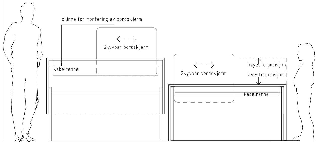
OPPRISS AA, PERSONALSIDE
