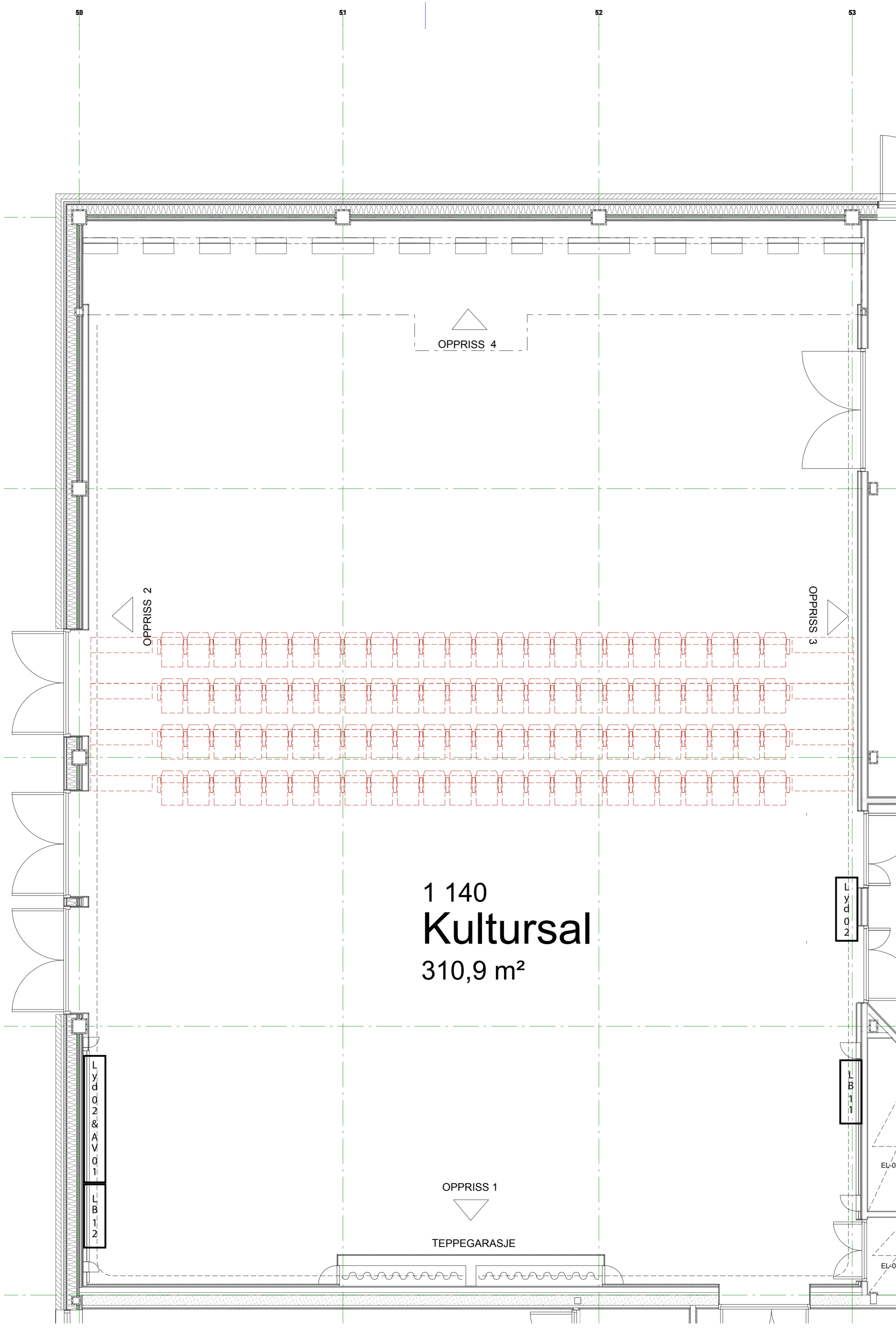
PLAN 1
