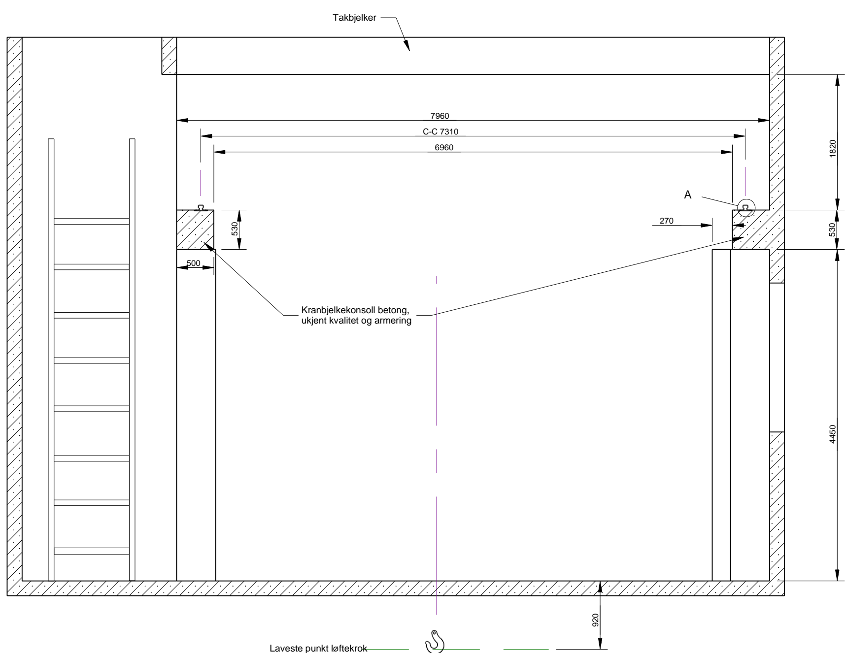
Section A-A (1:50)
