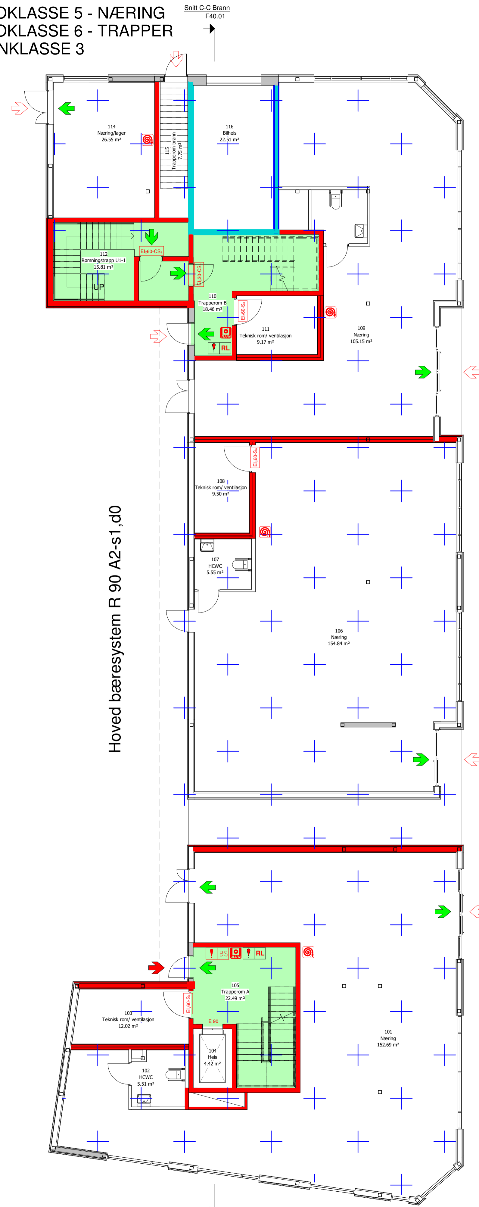
F25.01 Brannplan 1 1 : 100
