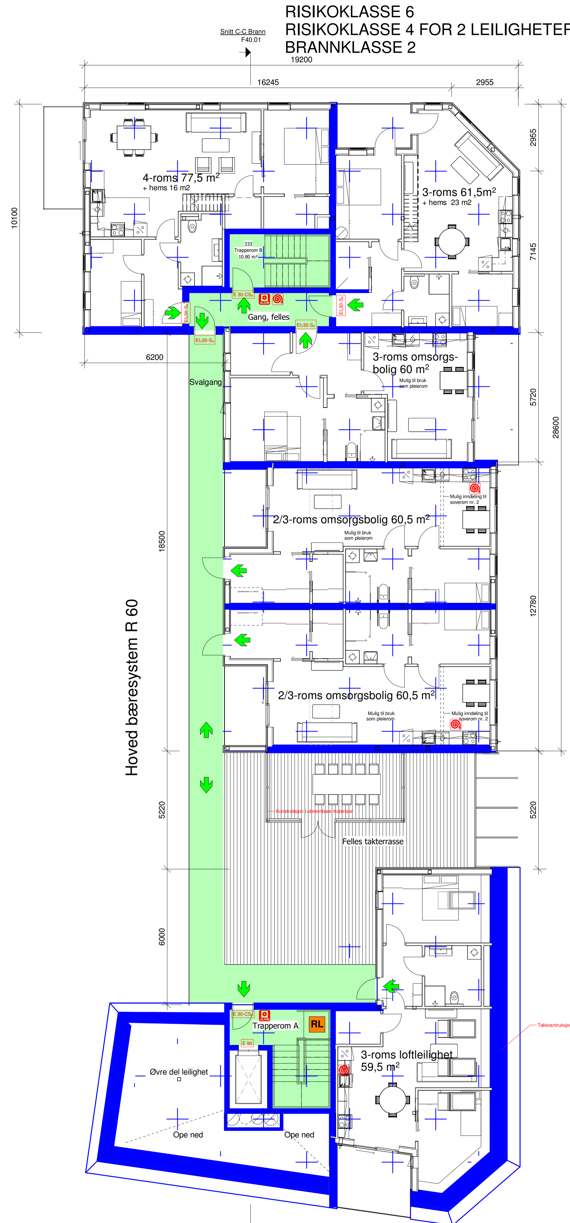
F25.03 Brannplan 3 1 : 100
