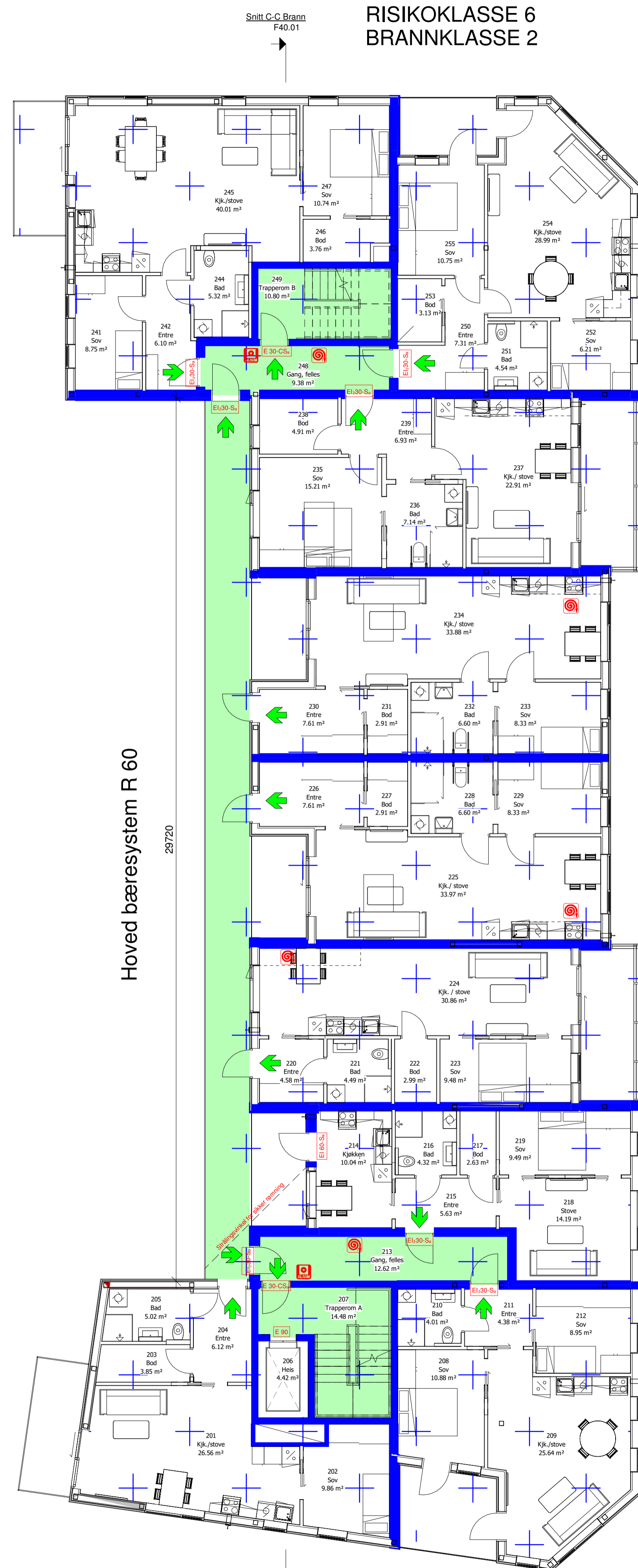
F25.02 Brannplan 2 1 : 100
