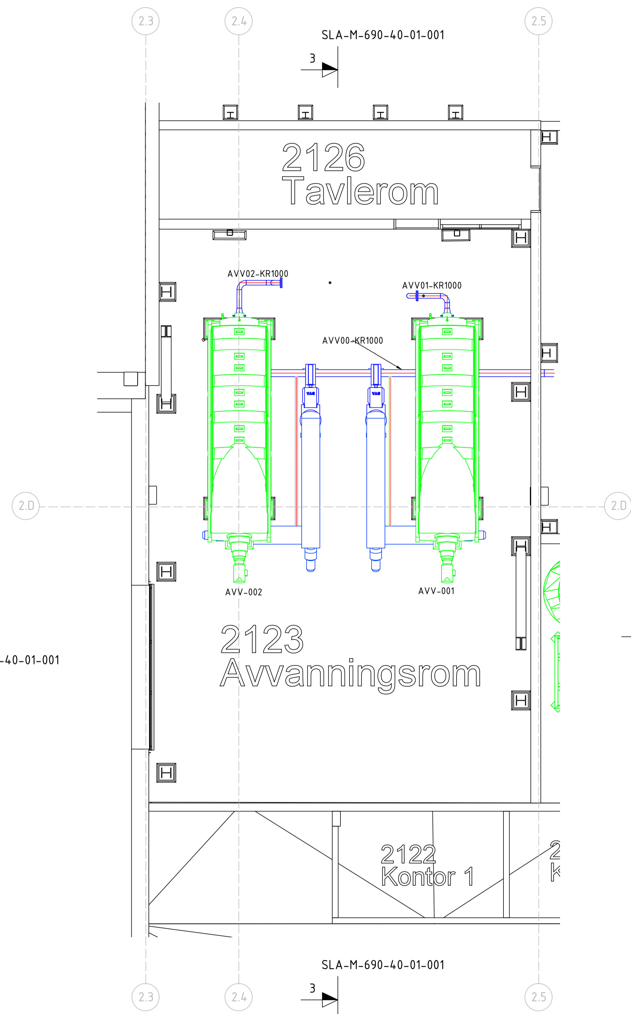
Plan 1 - Avvanningsrom k+1.0 1:50
