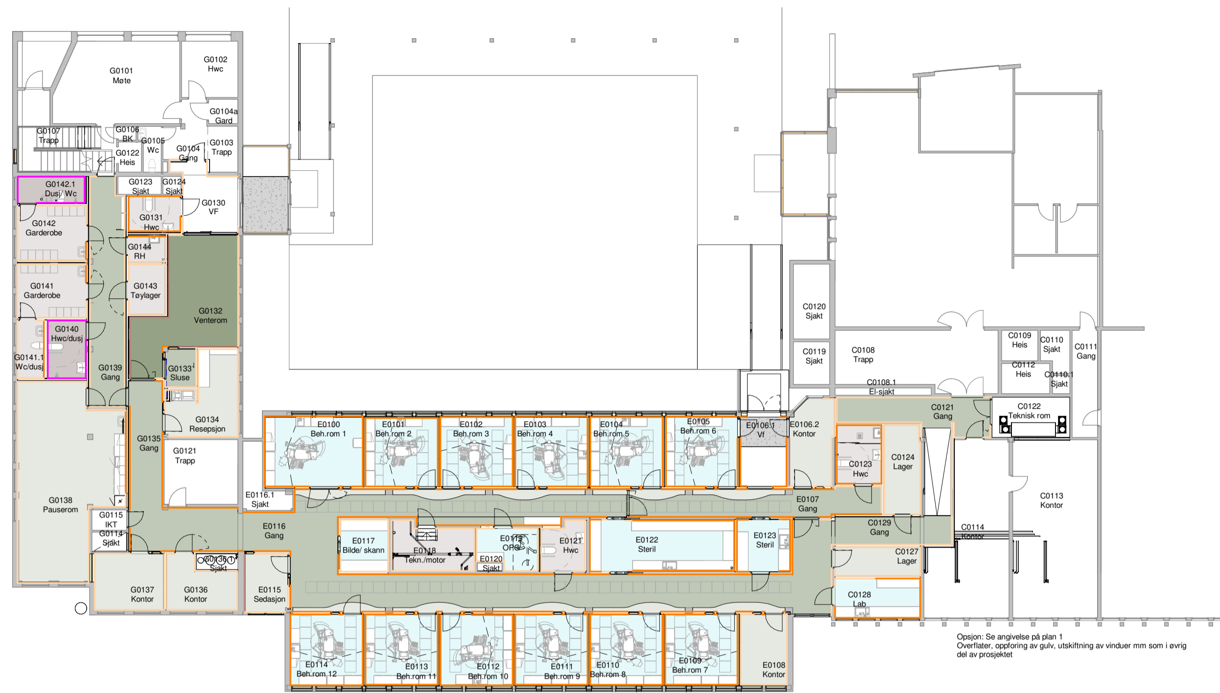
Plan 01 overflater vegg 1 : 200
