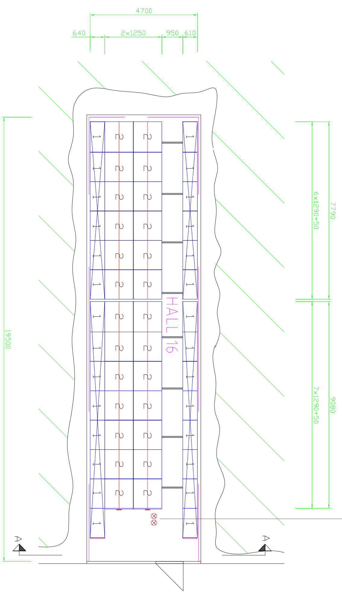
PLAN, HALL 16
