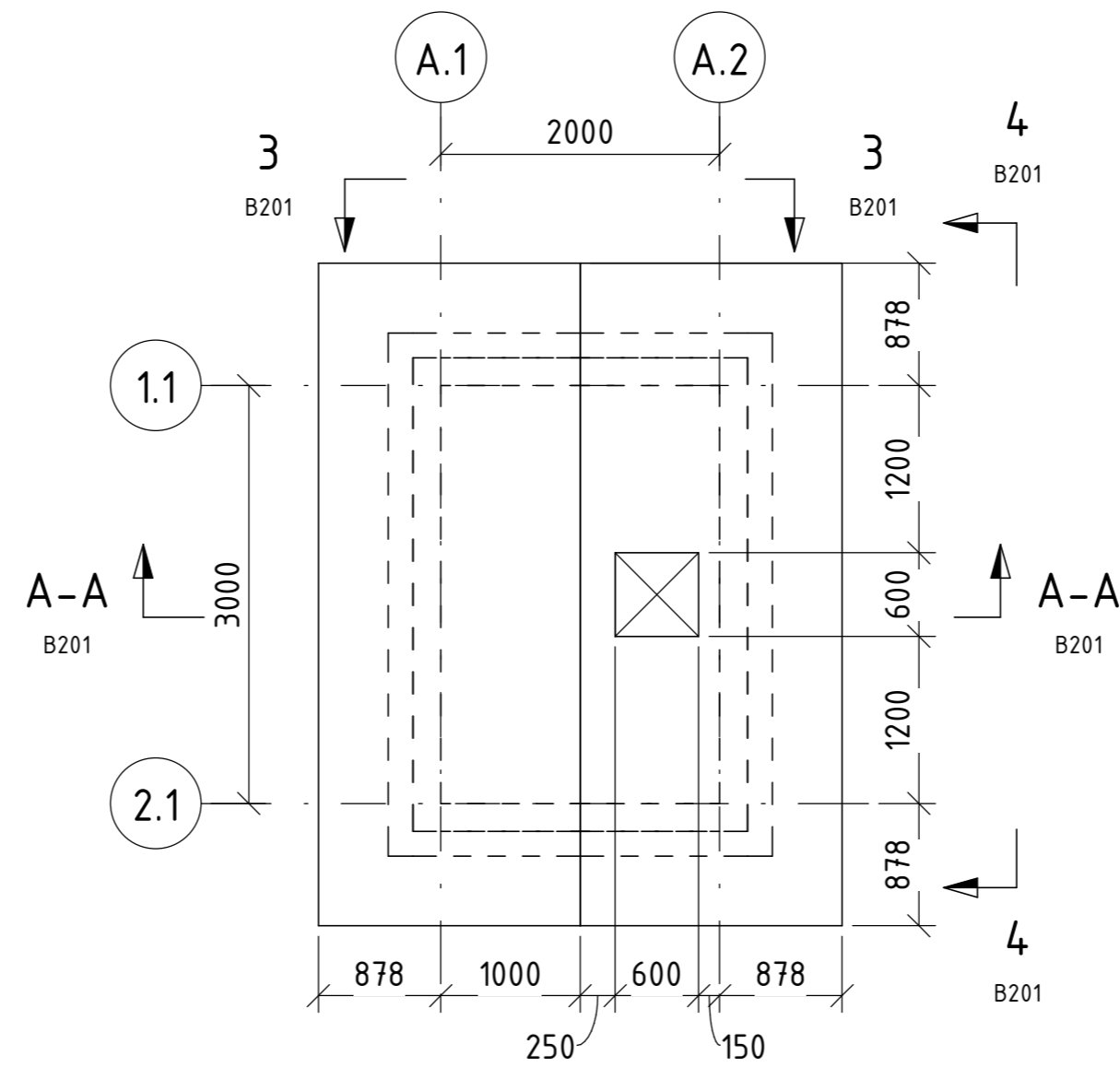
Takplan - Brønnhus 1 : 50
