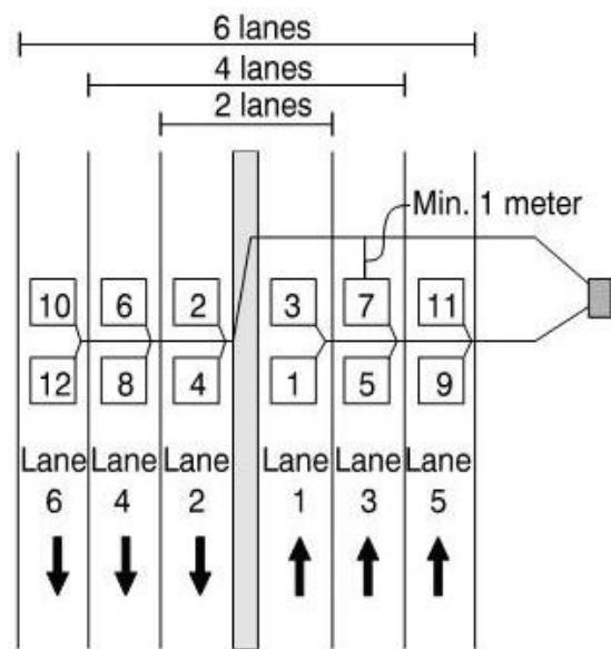
Figure 4 Example of typical loop configuration
