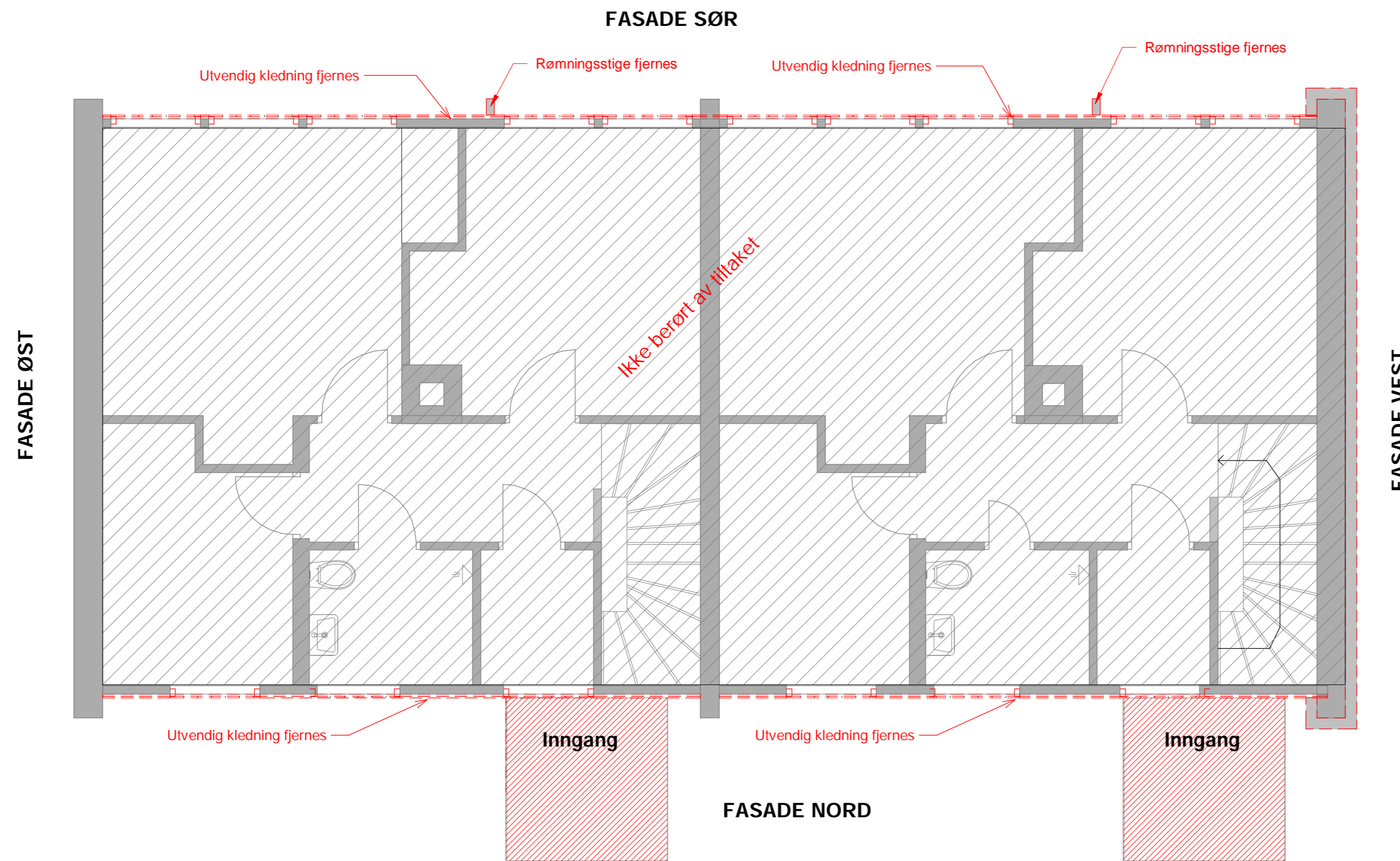
Plan 02_ Riveplan
