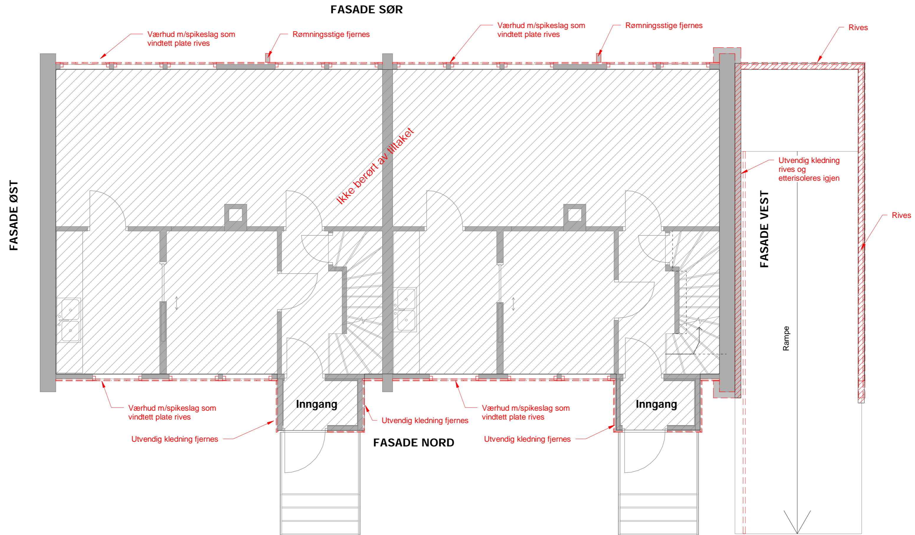
Plan 01_ Riveplan
