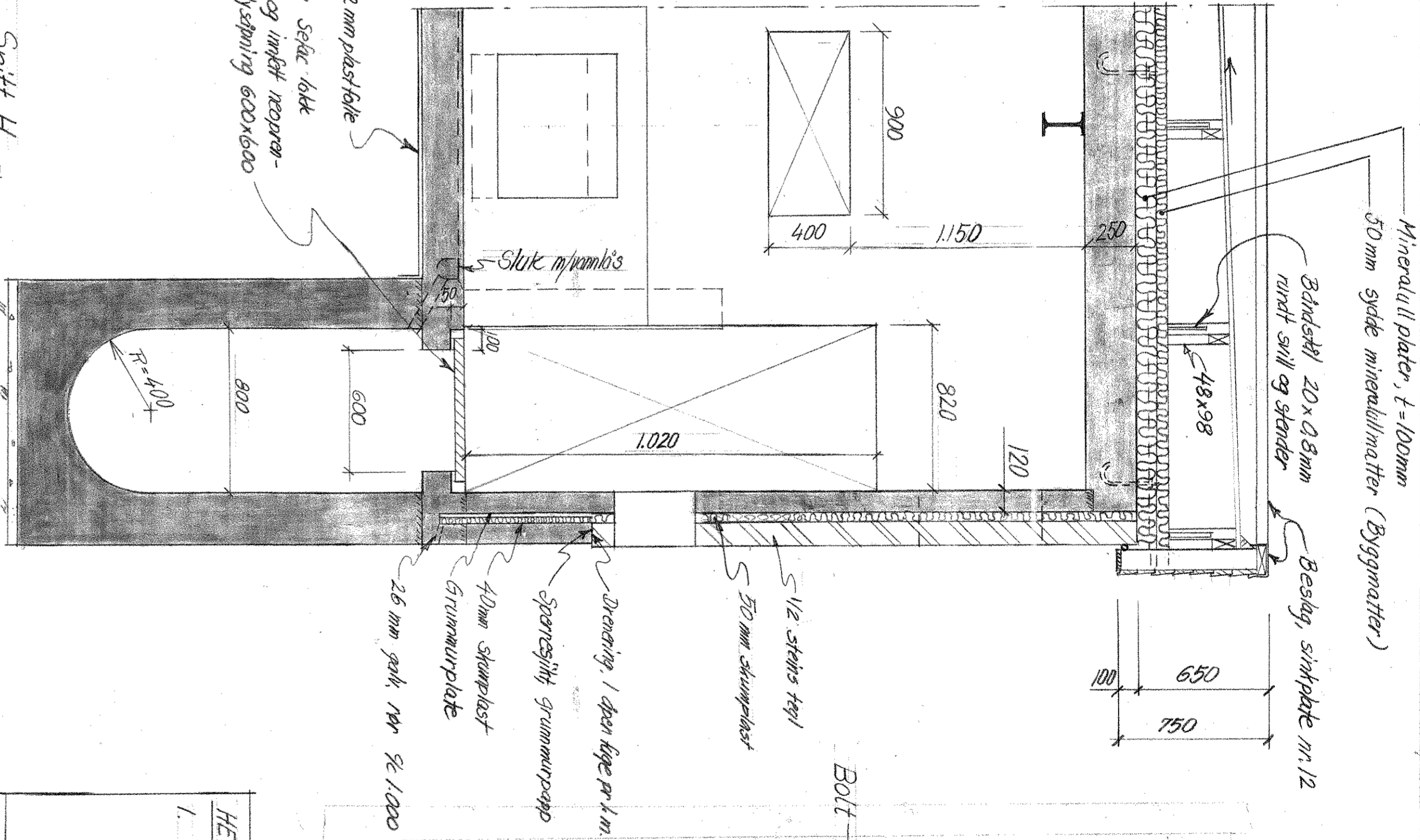
Takplan - betongtak 1:50
