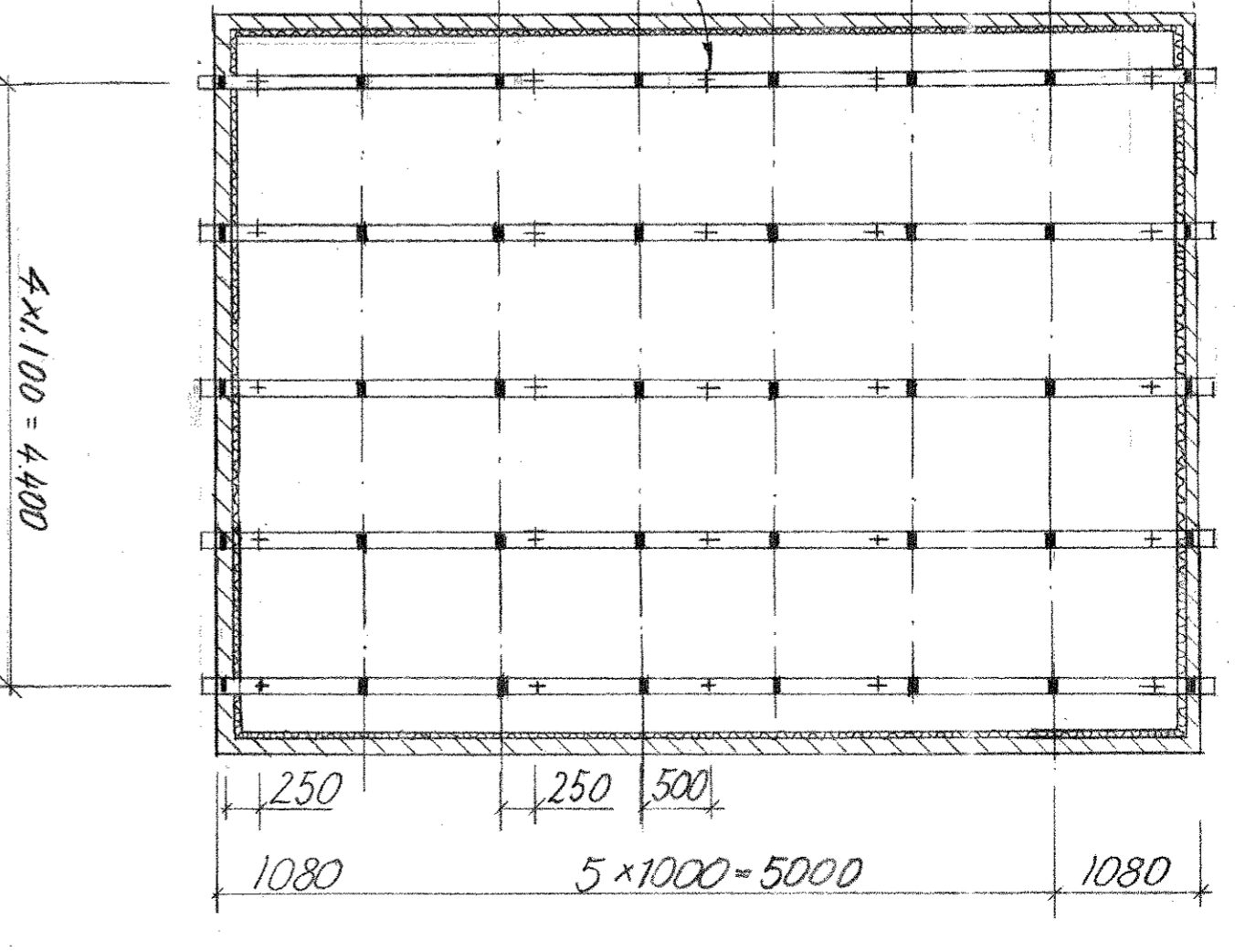
Takplan - betongtak 1:50
