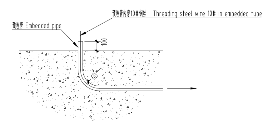
预埋管出地面工艺图 Diagram of Embedded pipe outside of the ground
