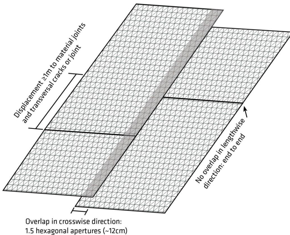
Figure 6: Overlap detail
