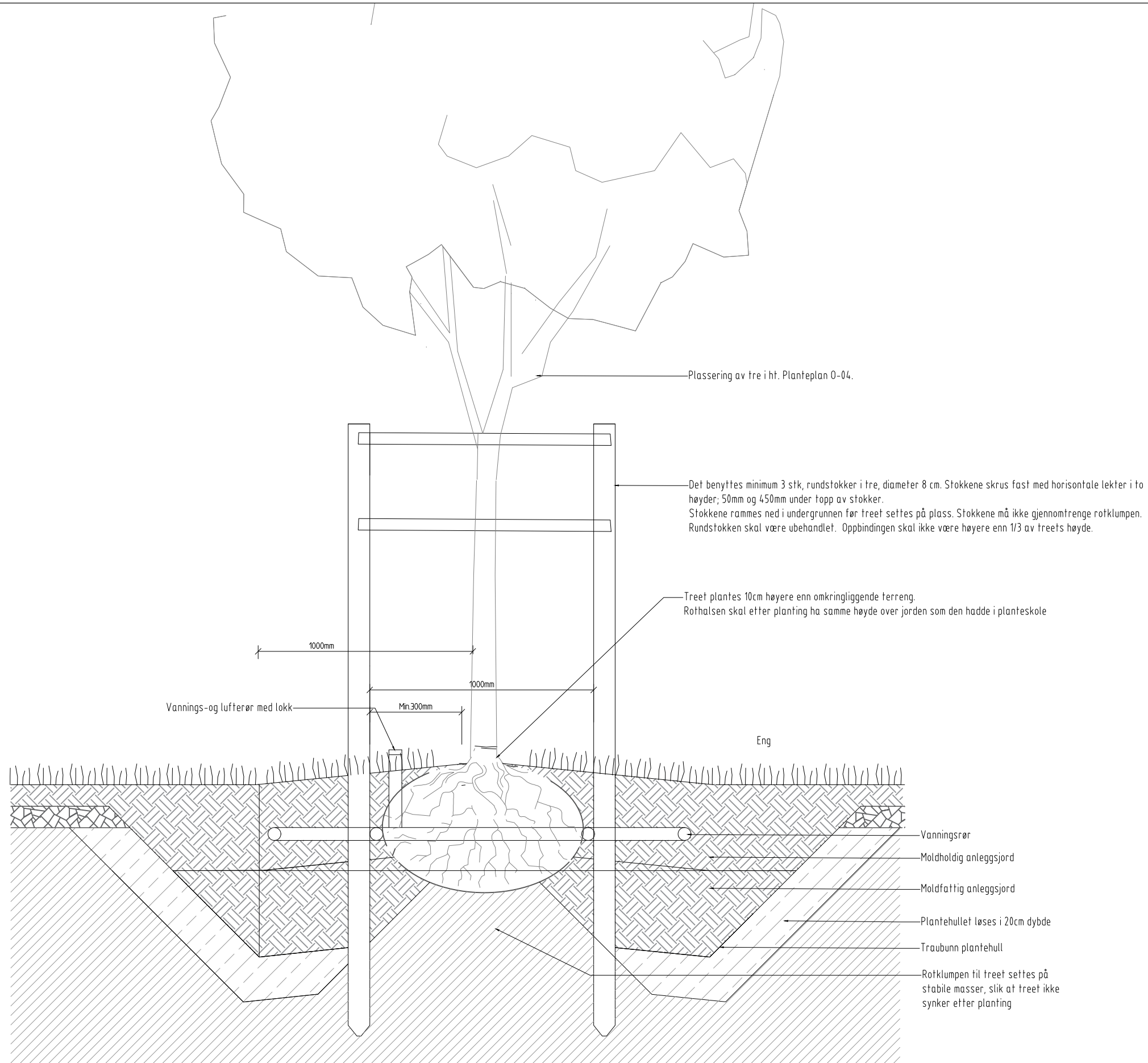
SNITT TREPLANTING
