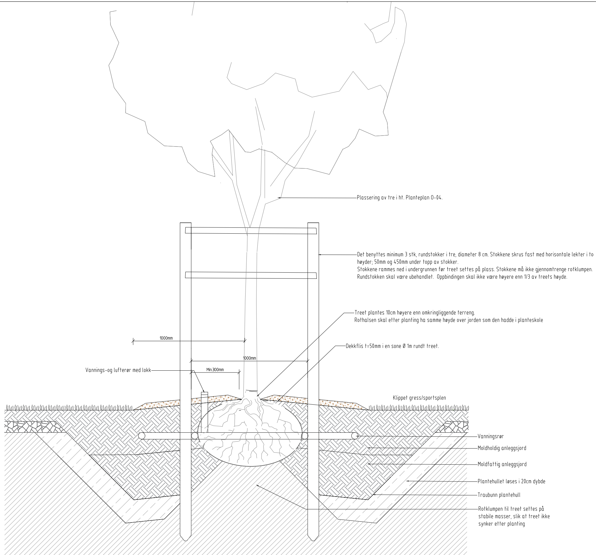
SNITT TREPLANTING
