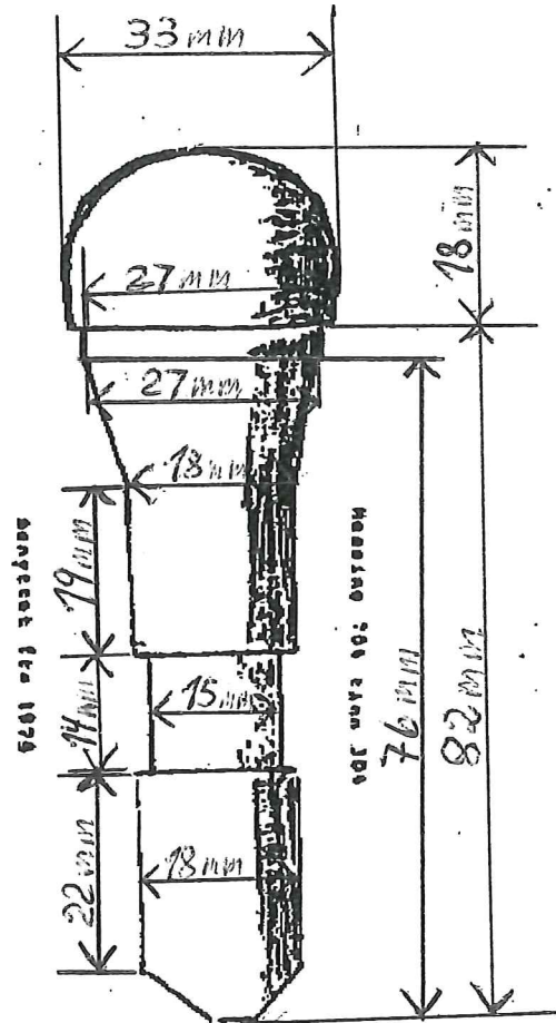
BOLT TYPE 7
