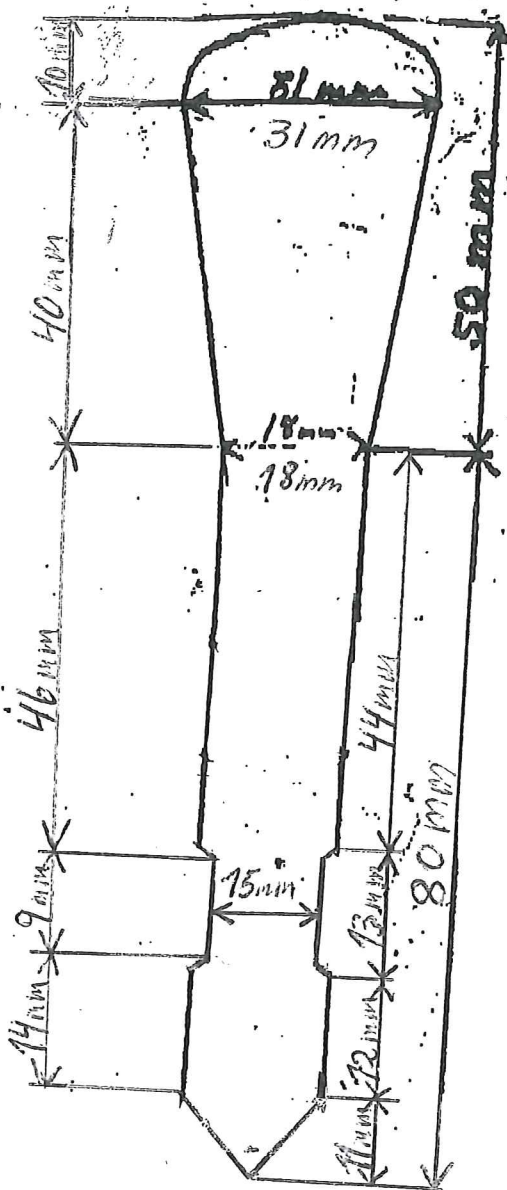
BOLT TYPE 2
