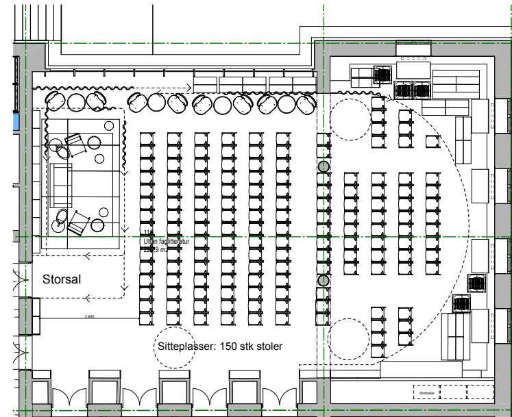
PLAN 1 1:200 STORSAL - FULL SAL
