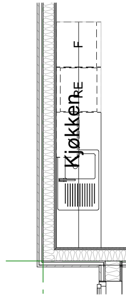
Leilighet 5: plan 1.50
