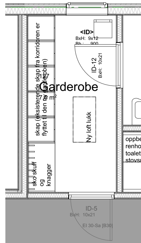
Garderobe - Plan
