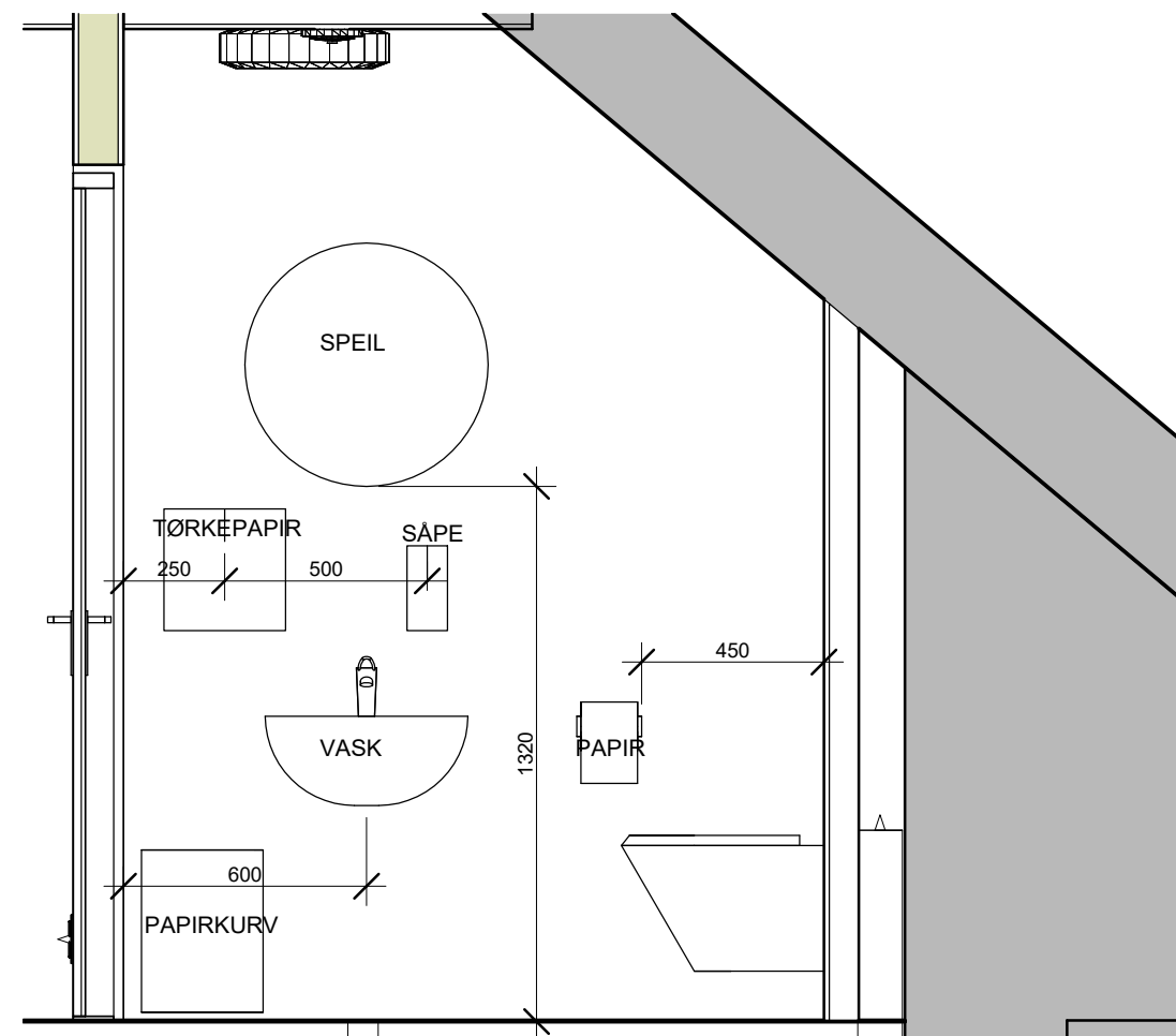
WC 2.04C OPPRISS 1 : 20
