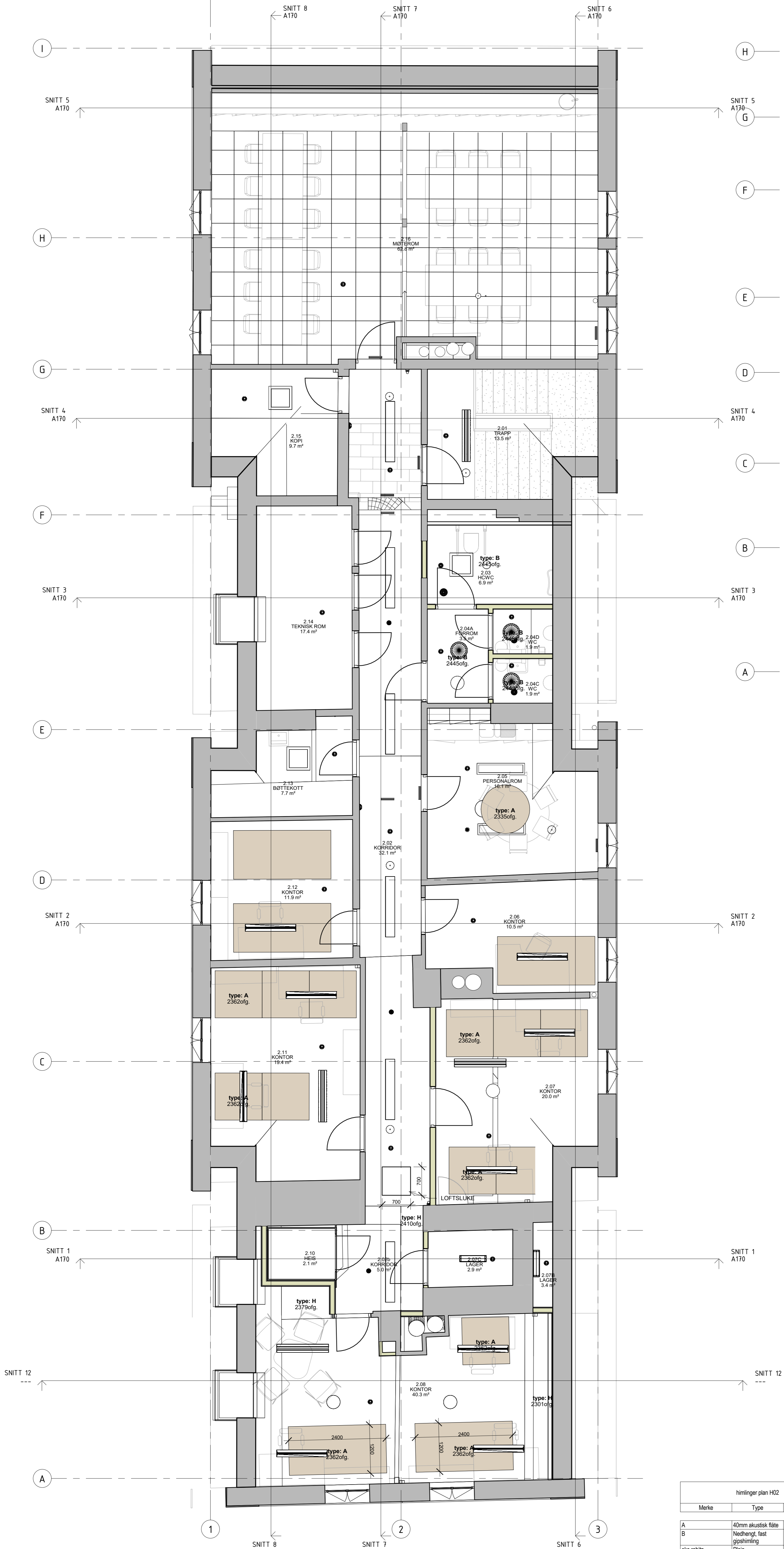
HIMLINGSPLAN H02 RIVING 1 : 100
