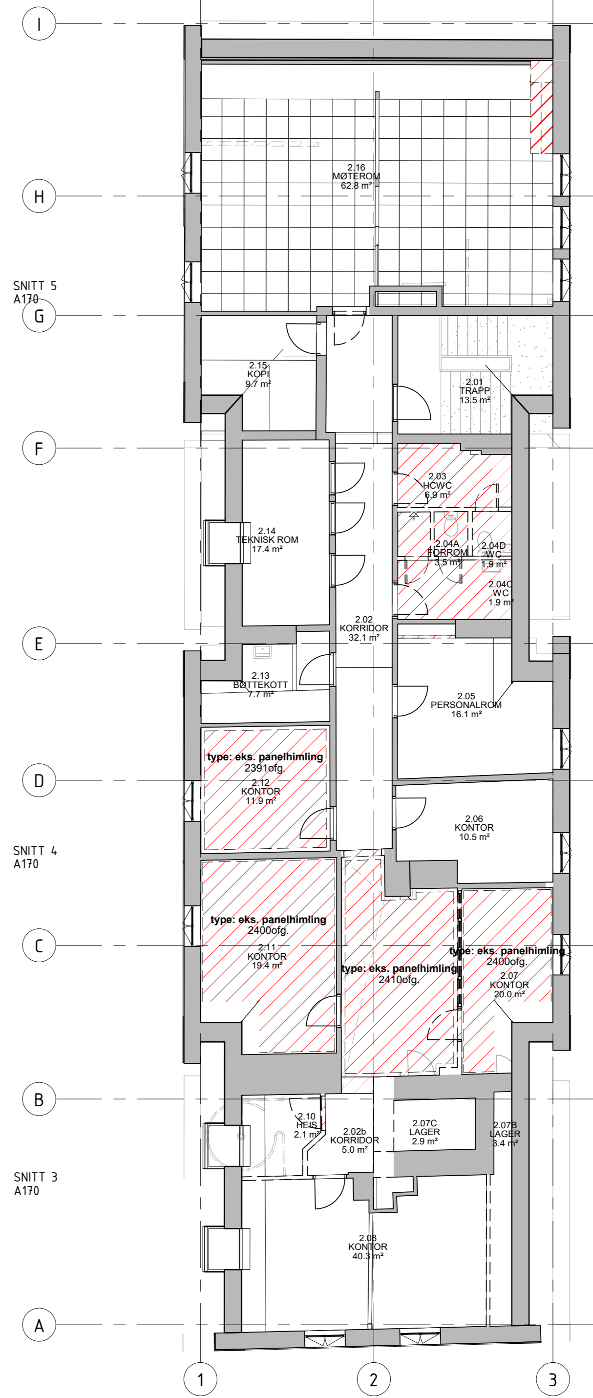
HIMLINGSPLAN H02 RIVING 1 : 100
