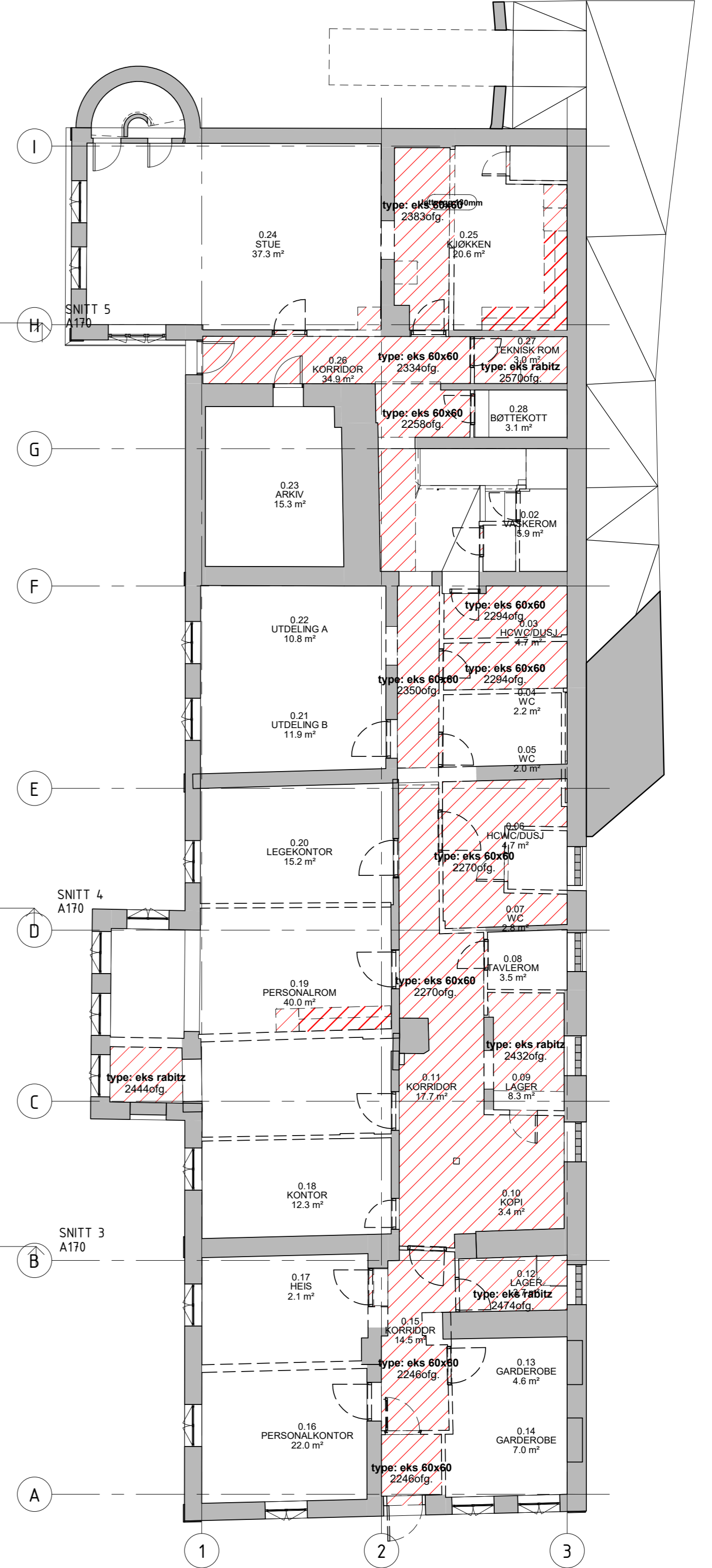
HIMLINGSPLAN U01, RIVING 1 : 100
