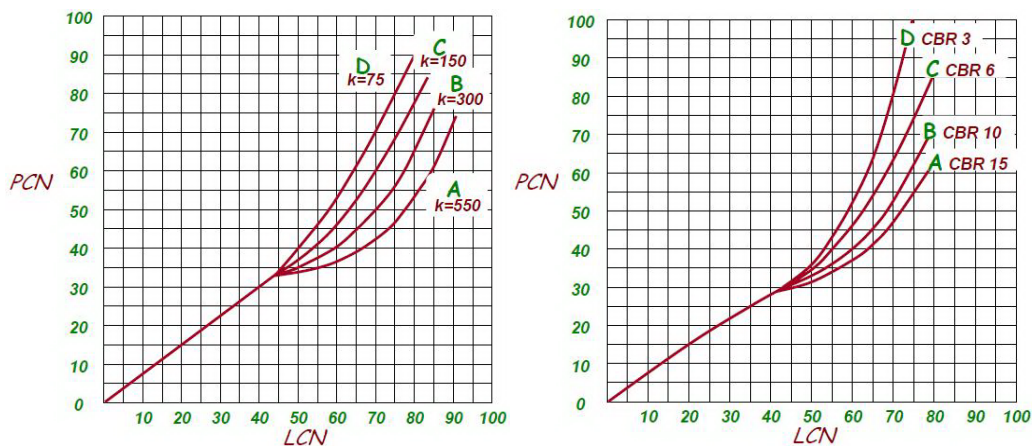
Figur 3-2 LCN-PCN
