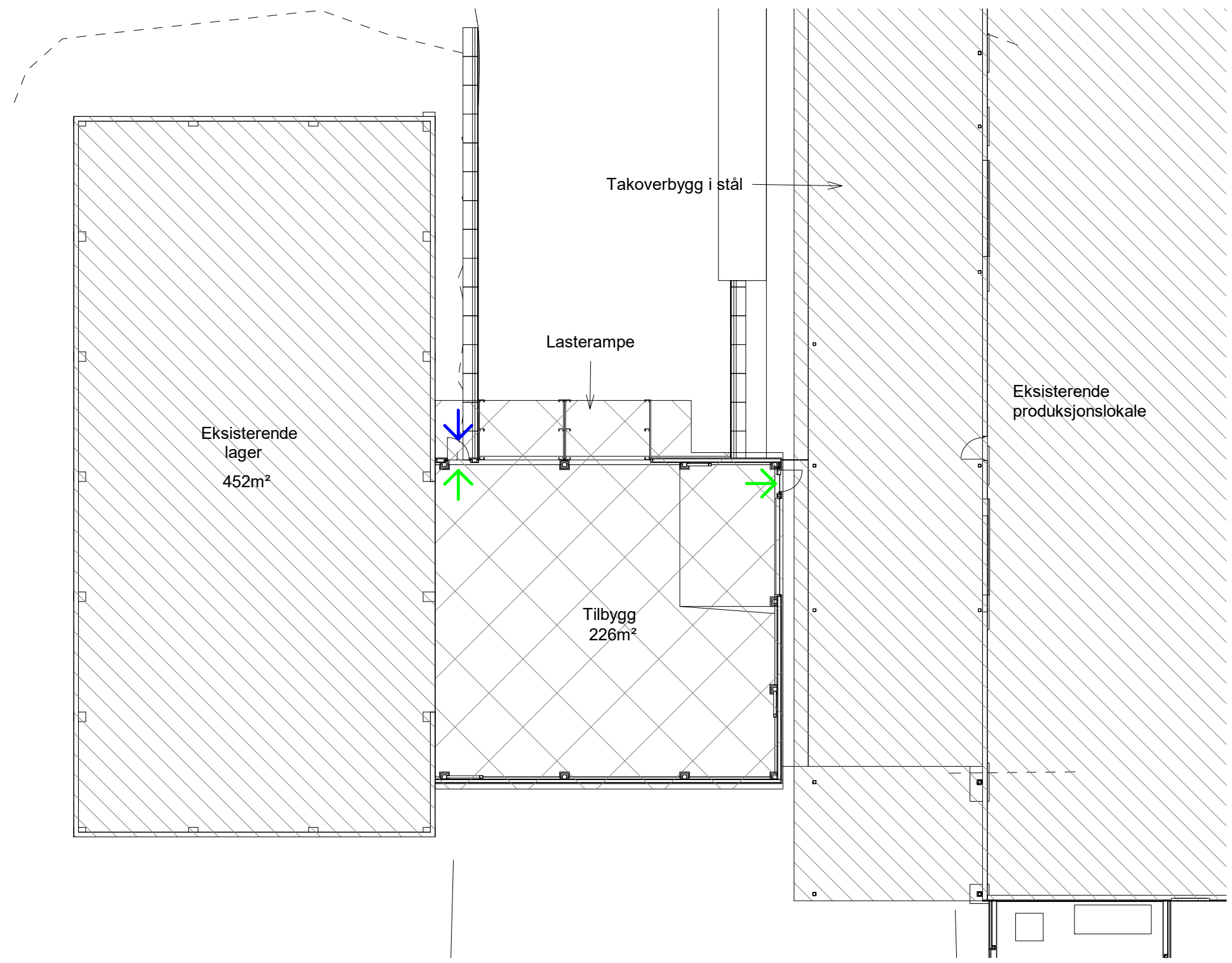
Brannplan 1 : 200
