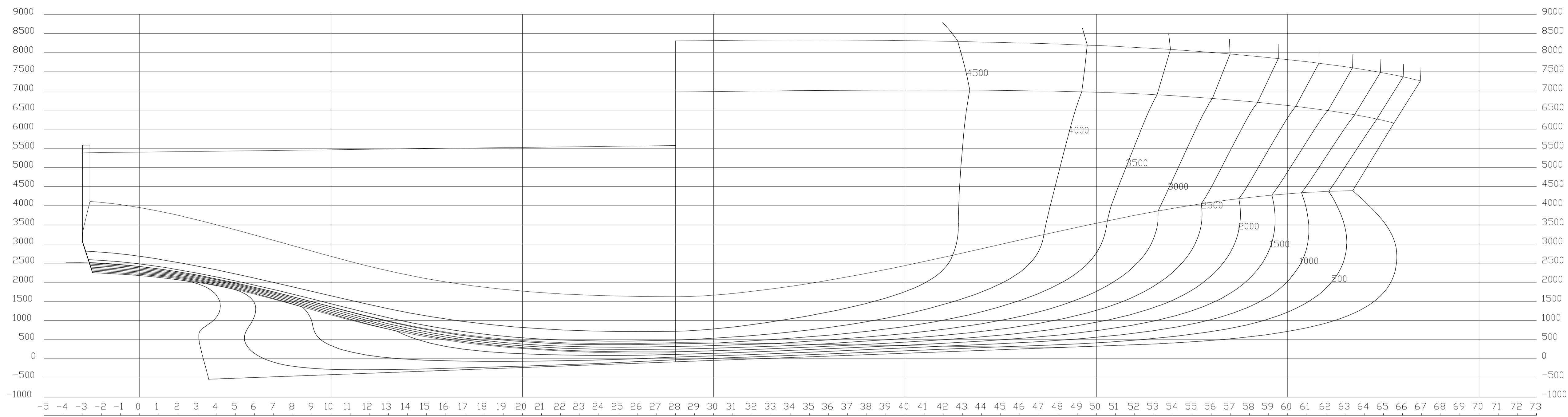
PROFILE & BUTTOCS VIEW
