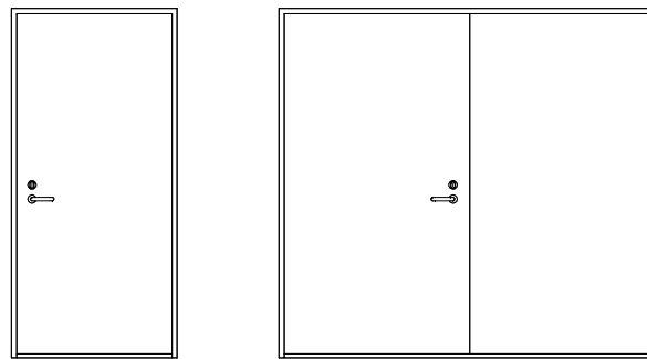
YD-40 10 x21M LYD: 37dB R'w+Ctr U-VERDI: 0,8 YD-41 23 x21M U-VERDI: 1,0
