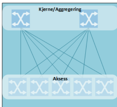
Figur 14 DC-LAN Spine/Leaf
