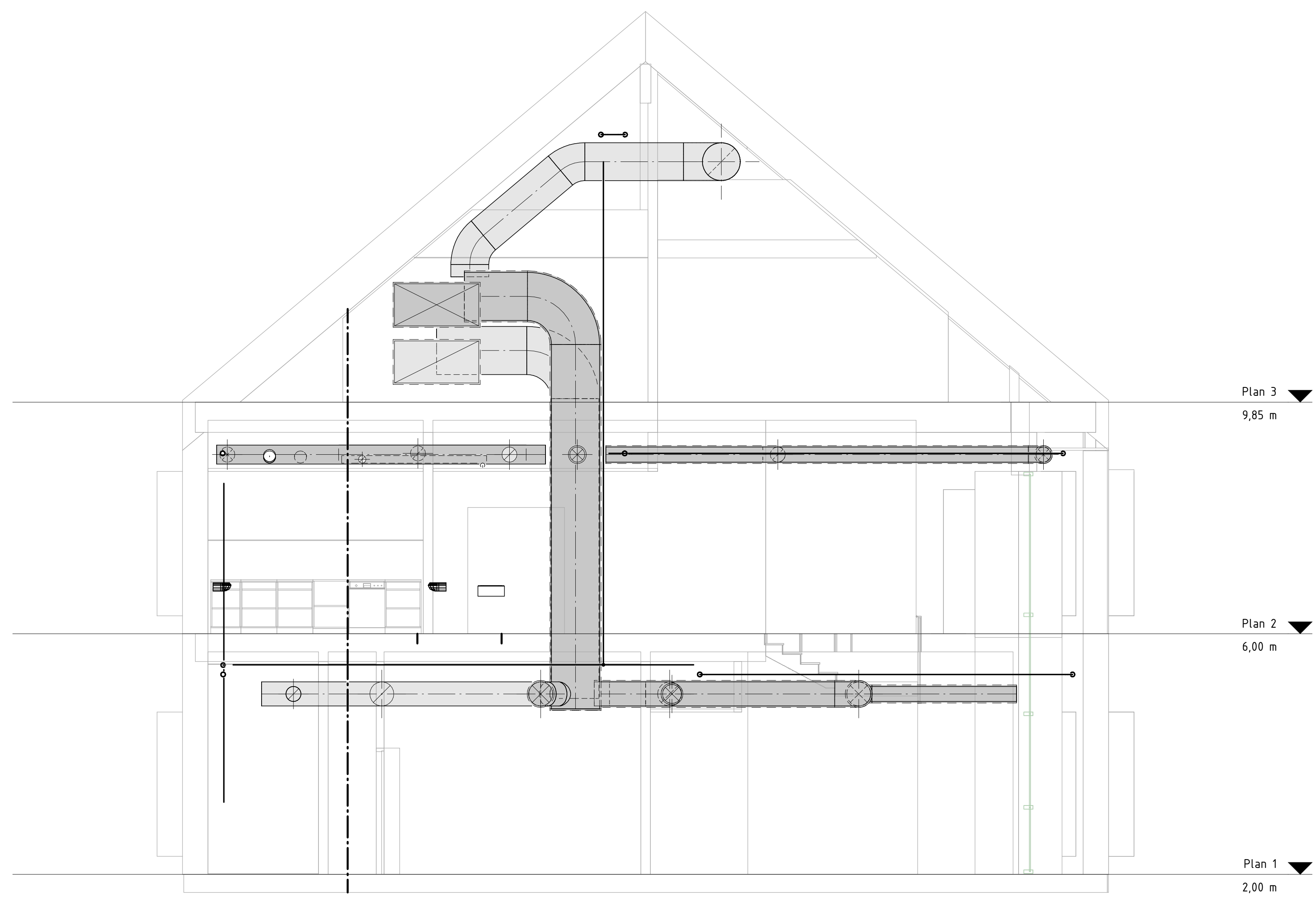
Section 1-1
