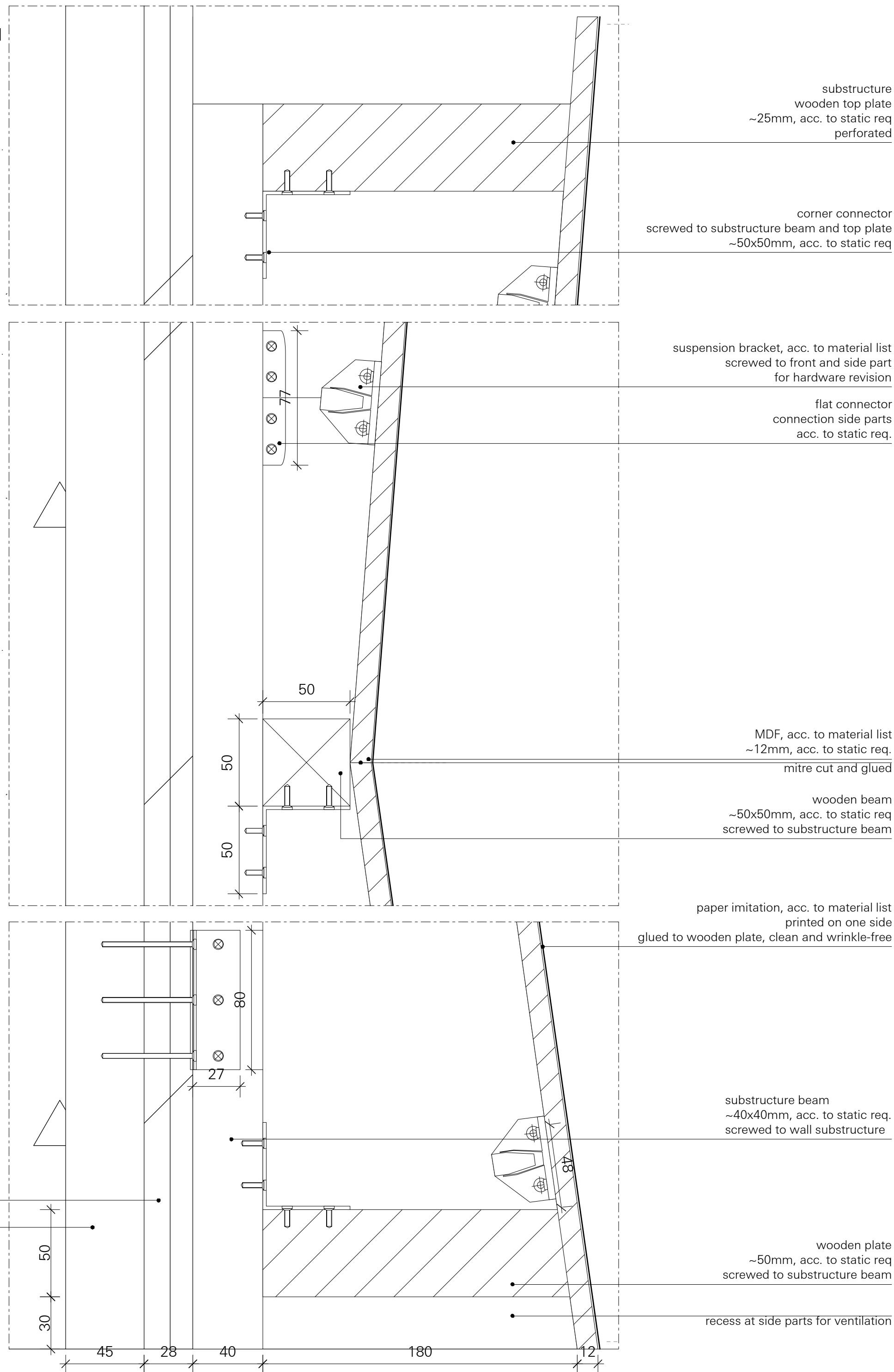
VERTICAL SECTION ANGLED WALL M 1:2
