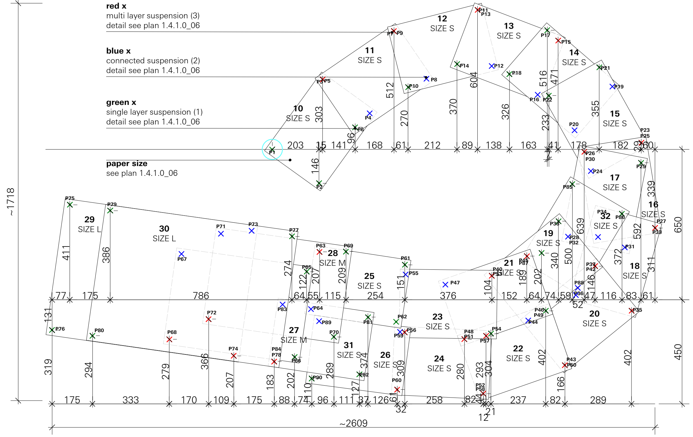
PAPER TWIST INSTALLATION TOP VIEW M 1:10
