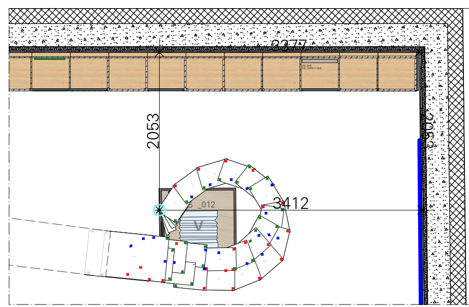
PAPER TWIST INSTALLATION SPACE REFERENCE M1:50
