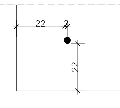
TOP VIEW SUSPENSION HOLE DETAIL M 1:1
