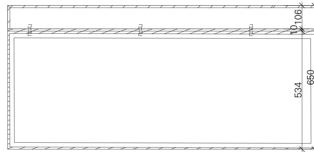
SHOWCASE HORIZONTAL SECTION C M 1:10
