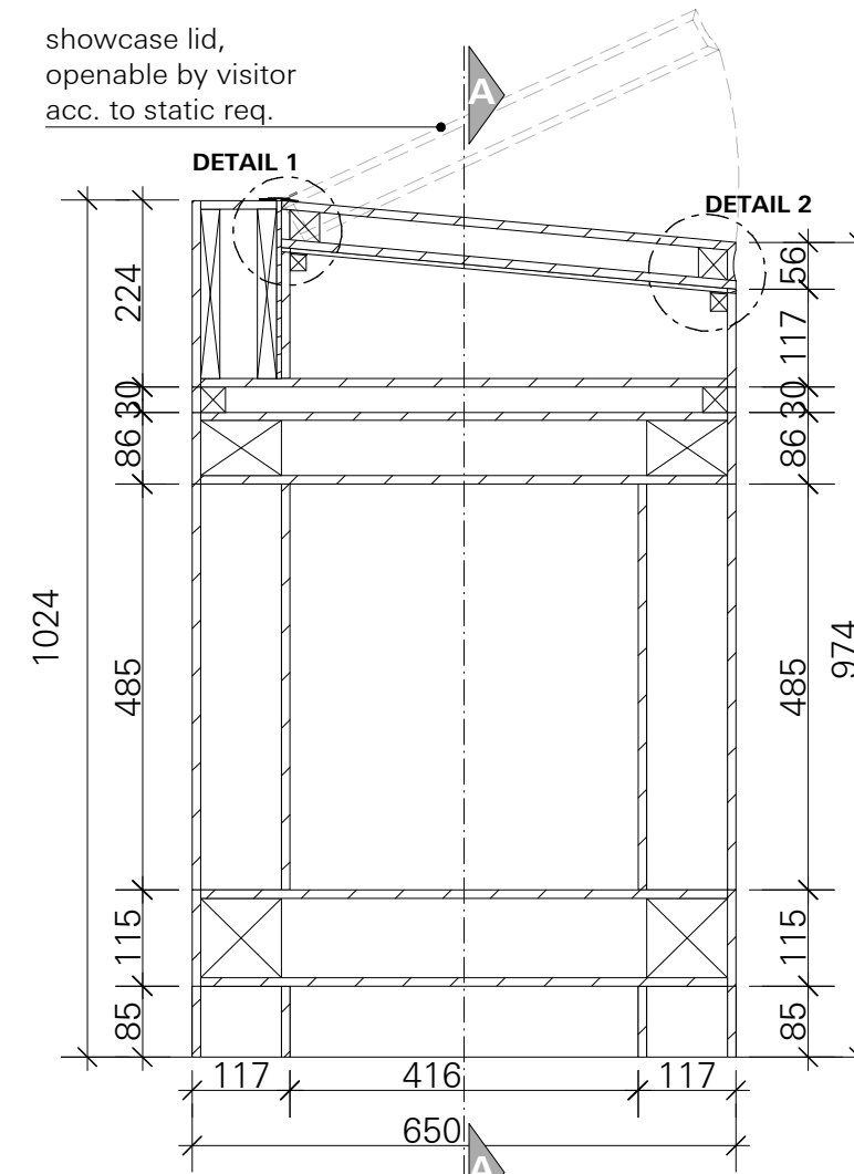
SHOWCASE VERTICAL SECTION B M 1:10
