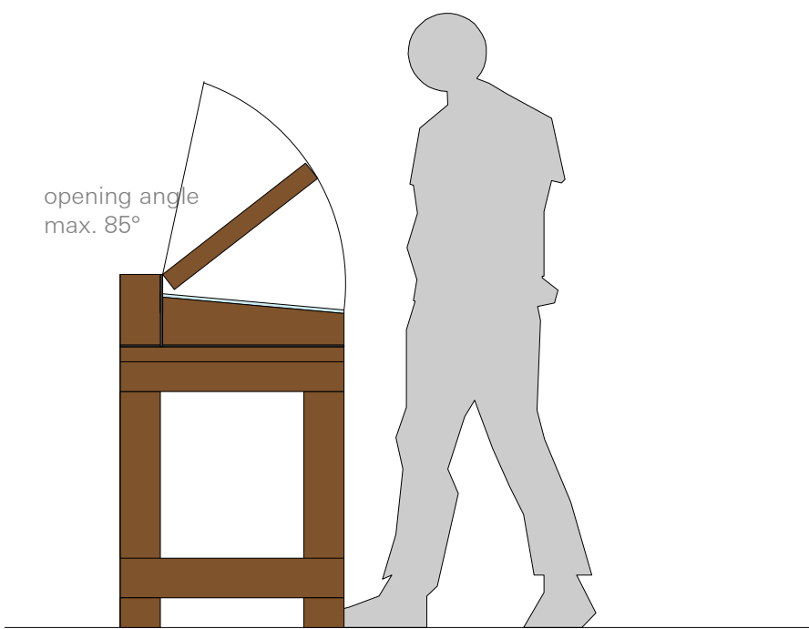
SHOWCASE SIDE VIEW M 1:20
