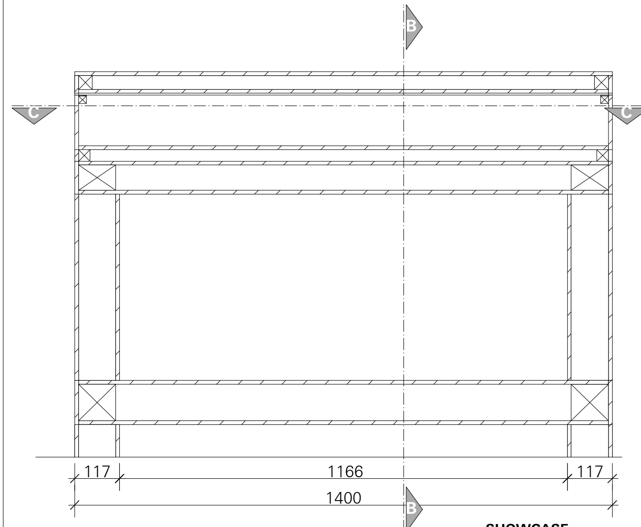
SHOWCASE VERTICAL SECTION A M 1:10
