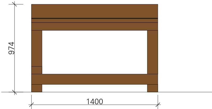
SHOWCASE FRONT VIEW M 1:20
