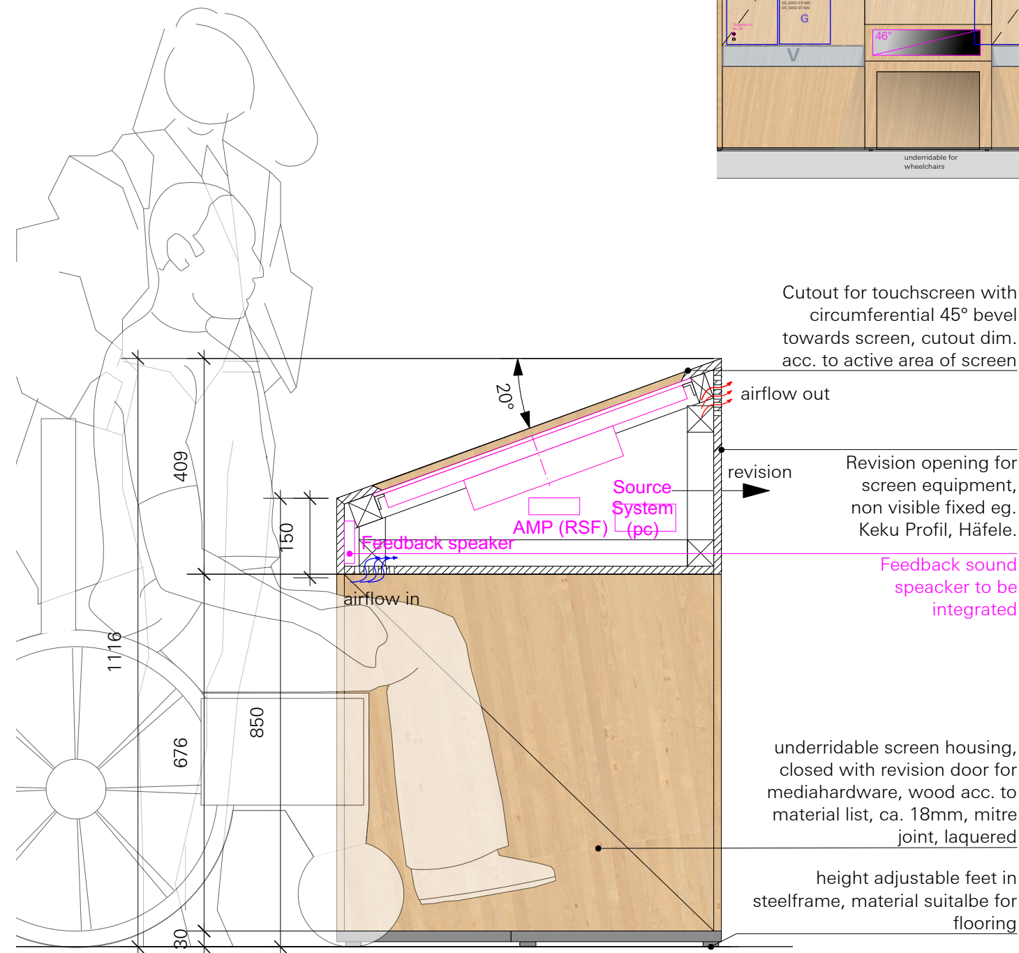
SECTION MEDIA STATION LABEL SHOWER MODULE E5 M 1:10
