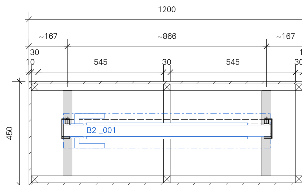
SECTION B MODULE B3b / C7 M 1:20
