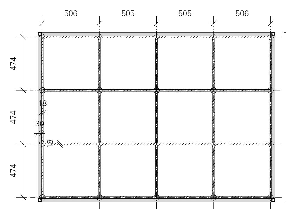
BASE SECTION HORIZONTAL MODULE C - GUTENBERGPRESS M 1:20
