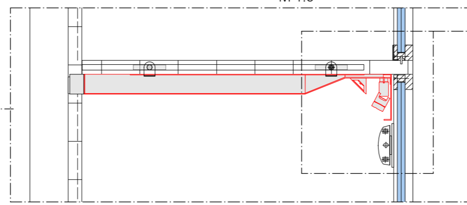
Lettercase Shelf Detail M 1:5
