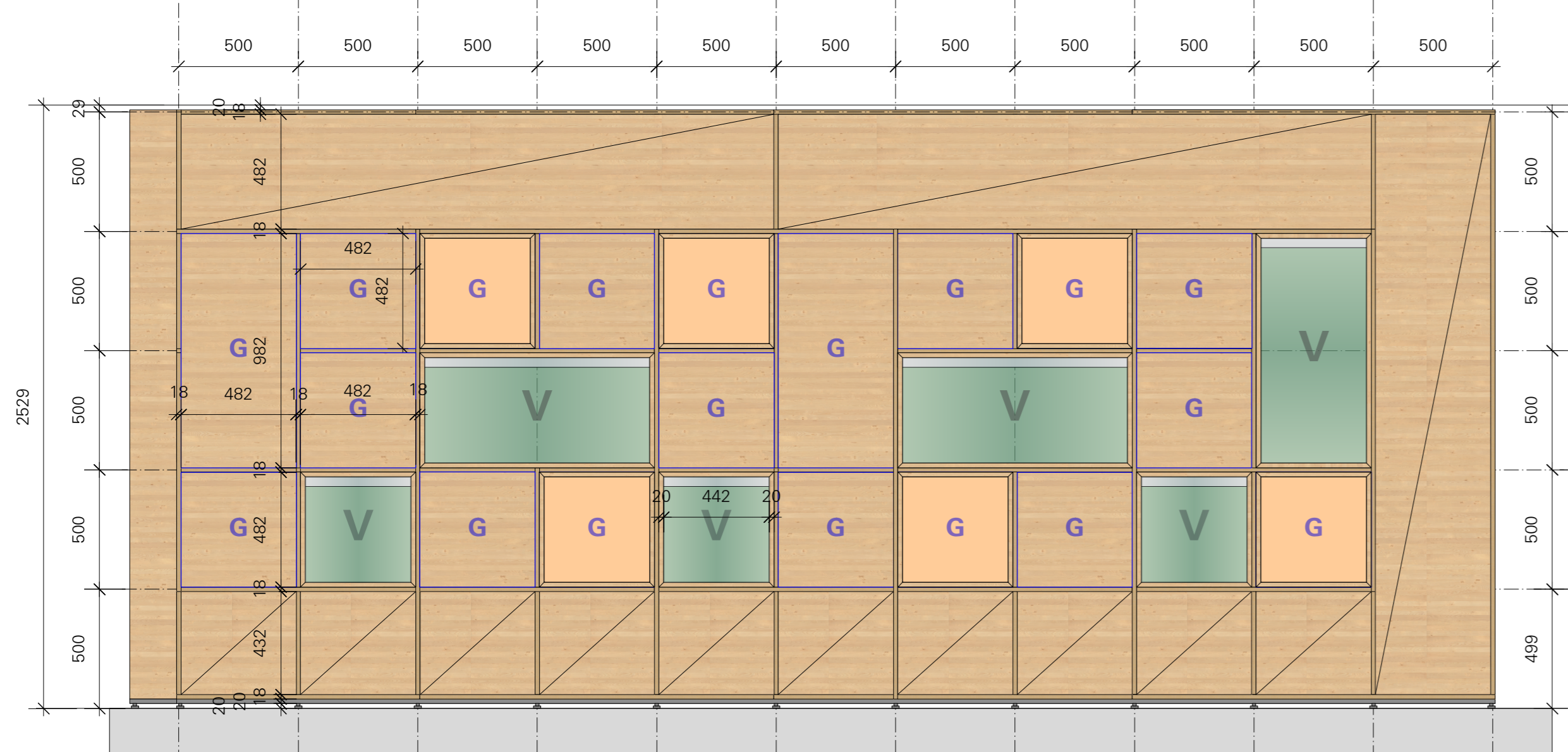
ELEVATION Lettercase Shelf full equipped with shelf components M 1:20
