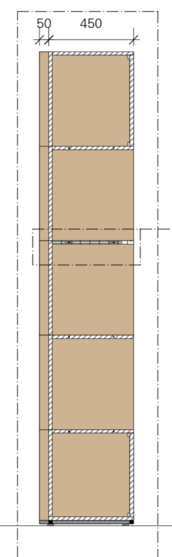
Lettercase Shelf section M 1:20
