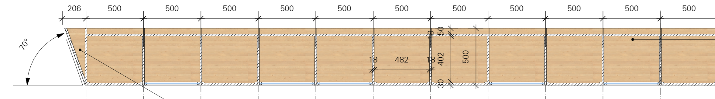
HORIZONTAL SECTION Lettercase Shelf full equipped with shelf components M 1:20
