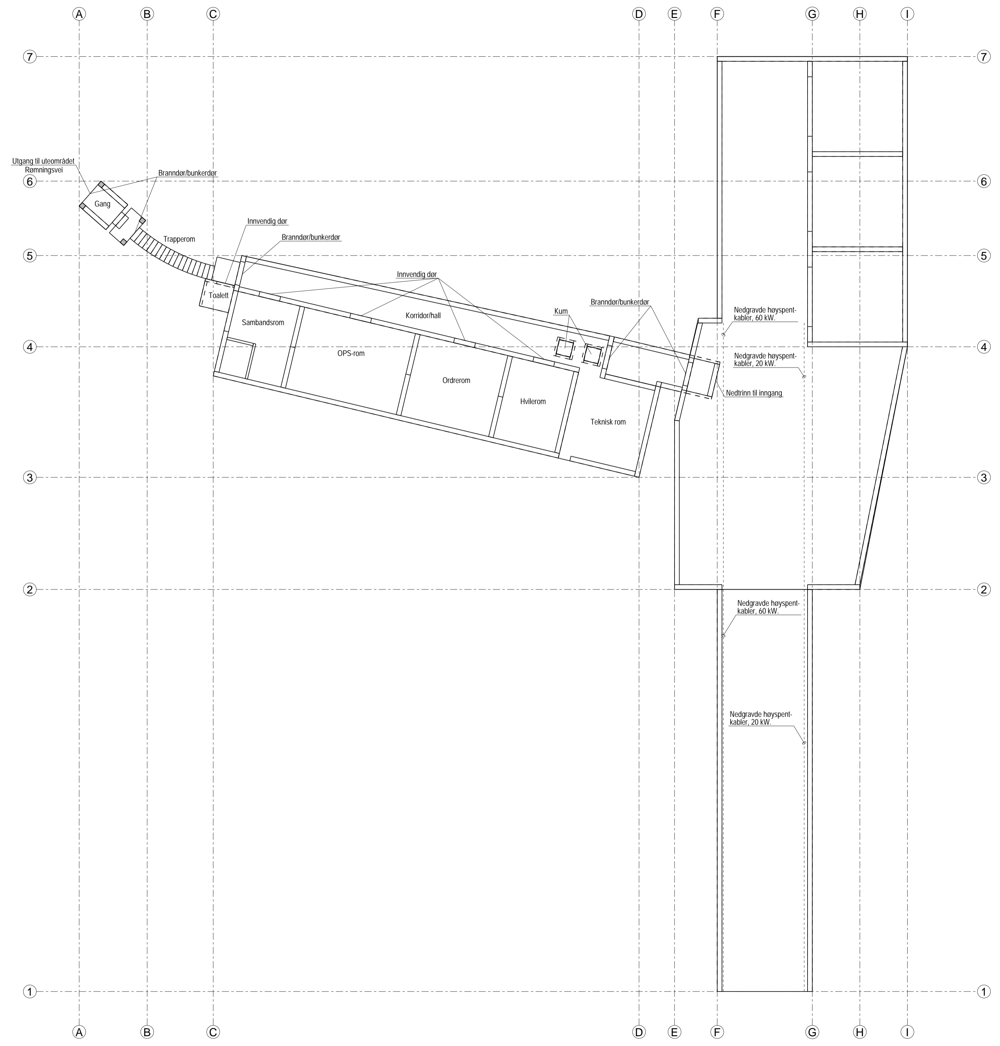
PLAN +0.00 1:100
